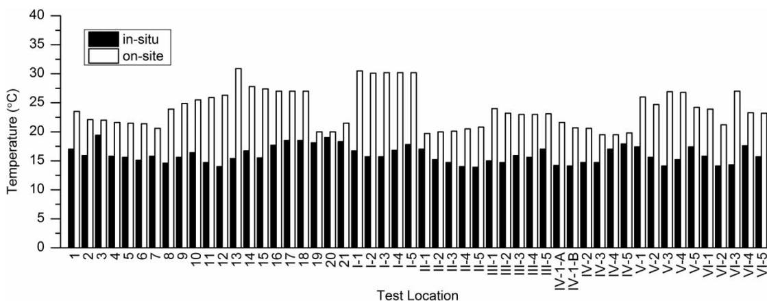
Figure 4 | Water temperatures at the 50 cm depth of streambed ( in situ ) and in the bucket (on-site) for the 52 pairs of tests.
