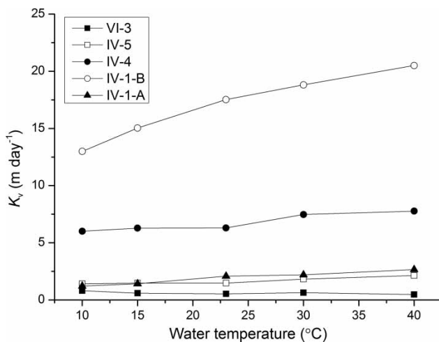
Figure 5 | Changes of K_v values with temperatures for five sediment cores.
