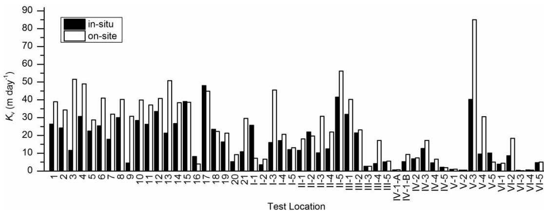
Figure 3 | K_v values from in situ permeameter tests and on-site permeameter tests at 52 locations.
