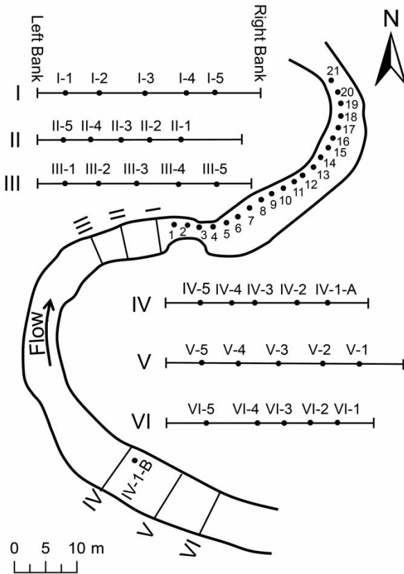
Figure 2 | Schematic of permeameter test locations.
