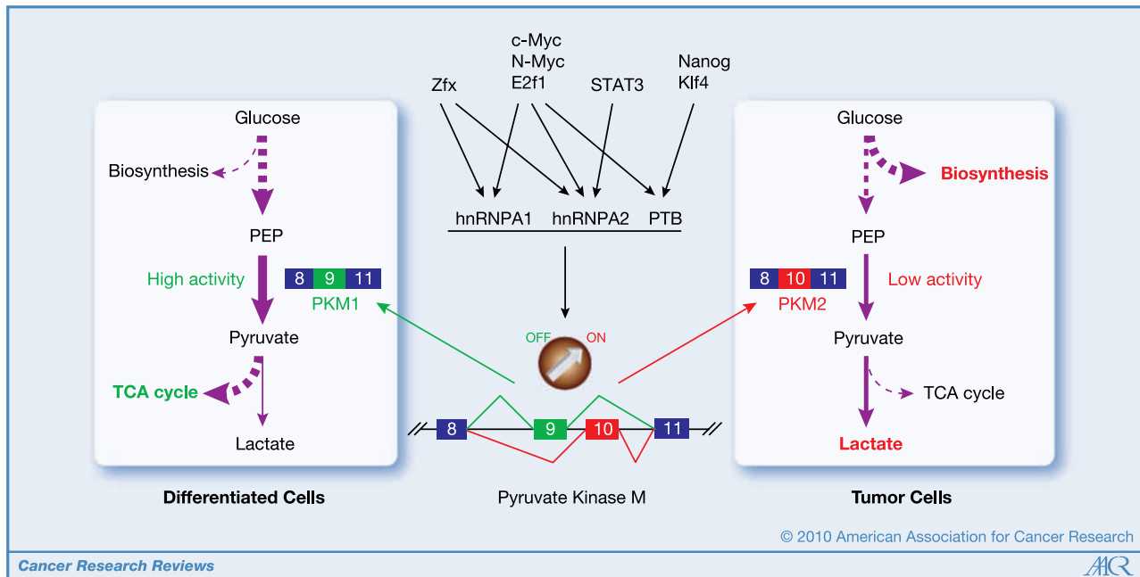
Figure 1. hnRNP proteins control the metabolic switch between oxidative phosphorylation and aerobic glycolysis by regulating the PKM alternative splicing. In cancer cells, transcription of hnRNPA1, A2, and PTB genes is upregulated, by c-Myc and, likely, one or more of the other factors indicated. Binding of the hnRNPs to the splice sites flanking exon 9 in PKM transcripts results in exon 9 exclusion and exon 10 inclusion, generating PKM2. PKM2 converts PEP to pyruvate less efficiently than PKM1, leading to the accumulation of glycolytic metabolites for anabolic metabolism (efficiencies indicated by thickness of arrows).
