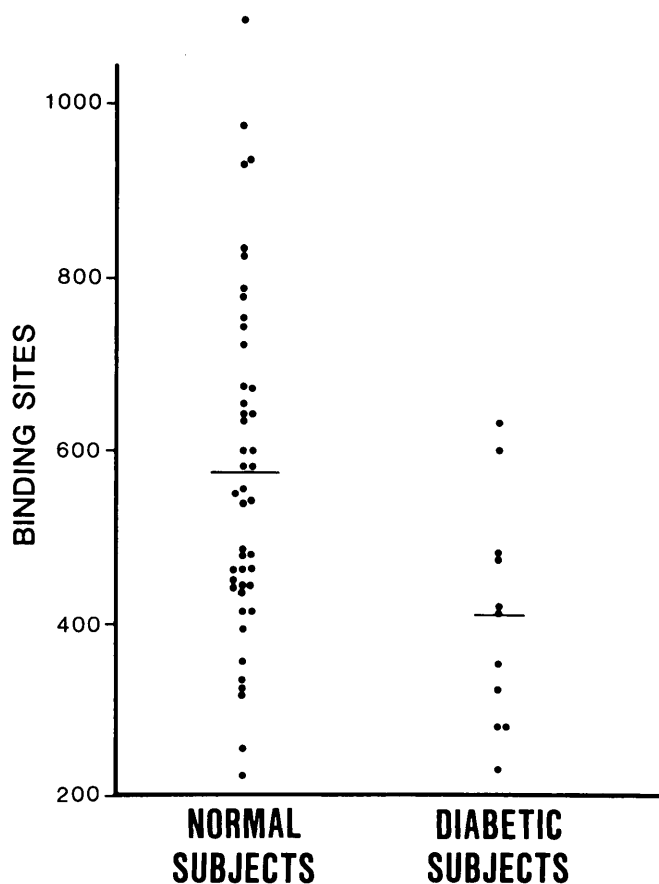
FIG. 1. Number of binding sites per platelet for normal ( 574 \pm 29 SEM) and diabetic ( 430 \pm 40 SEM) subjects is shown. The 2 groups were statistically different at P = .005 .
