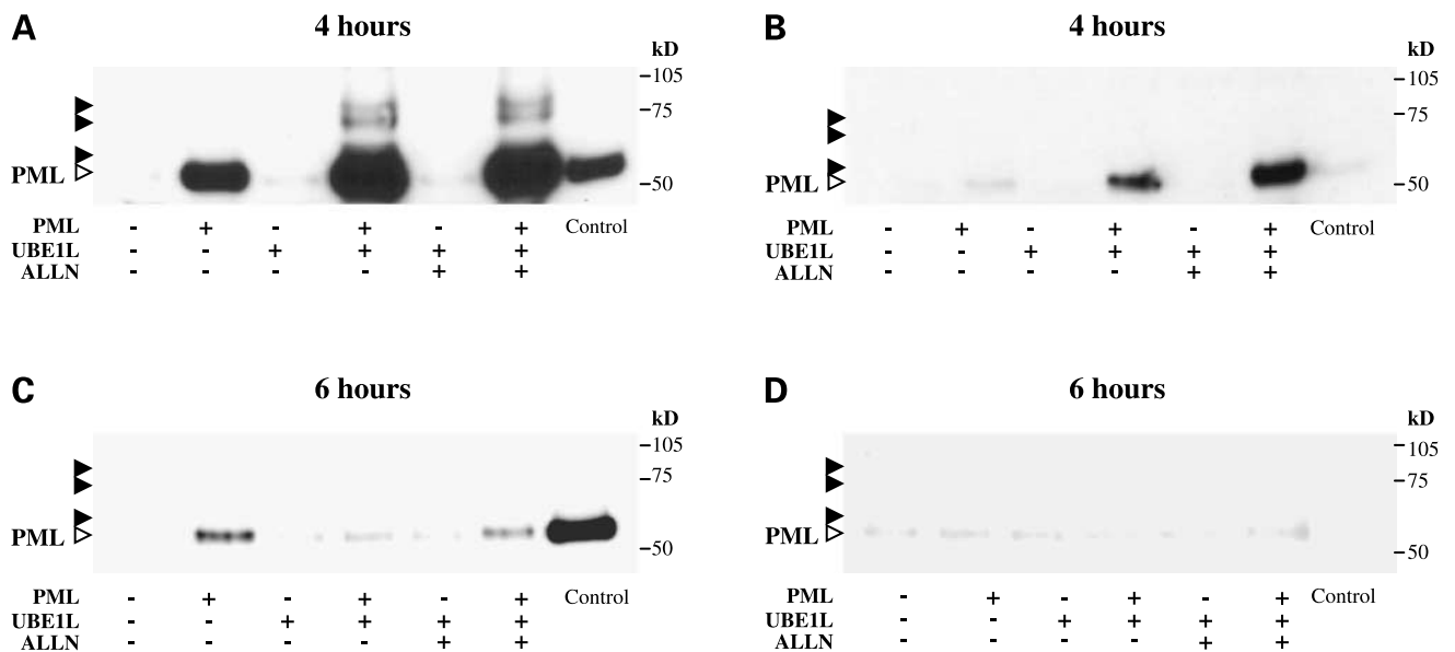
Figure 6. Effects of UBE1L on ISG15ylation of the PML domain of PML/RAR \alpha . BEAS-2B cells were individually transfected with the PML domain fragment of PML/RAR \alpha containing expression construct. Indicated groups were cotransfected with or without UBE1L. Following transfection, respective groups were treated with either ALLN (100 \mu mol/L) or vehicle (DMSO) for 4 ( A and B ) or 6 ( C and D ) additional hours. Immunoprecipitation followed by immunoblot analyses were done as described in Materials and Methods. The filters were probed with either a monoclonal anti-HA antibody to detect PML ( A and C ) or a monoclonal anti-ISG15 antibody to detect ISG15ylated forms of PML ( B and D ). Open arrows , positions of unconjugated PML protein; closed arrows , positions of post-translational modification products; Control , whole-cell lysates of COS-1 cells transfected with PML serve as a signal for the unconjugated form of PML. These experiments established that UBE1L confers ISG15 conjugation to the PML domain of PML/RAR \alpha with subsequent repression of this protein.
