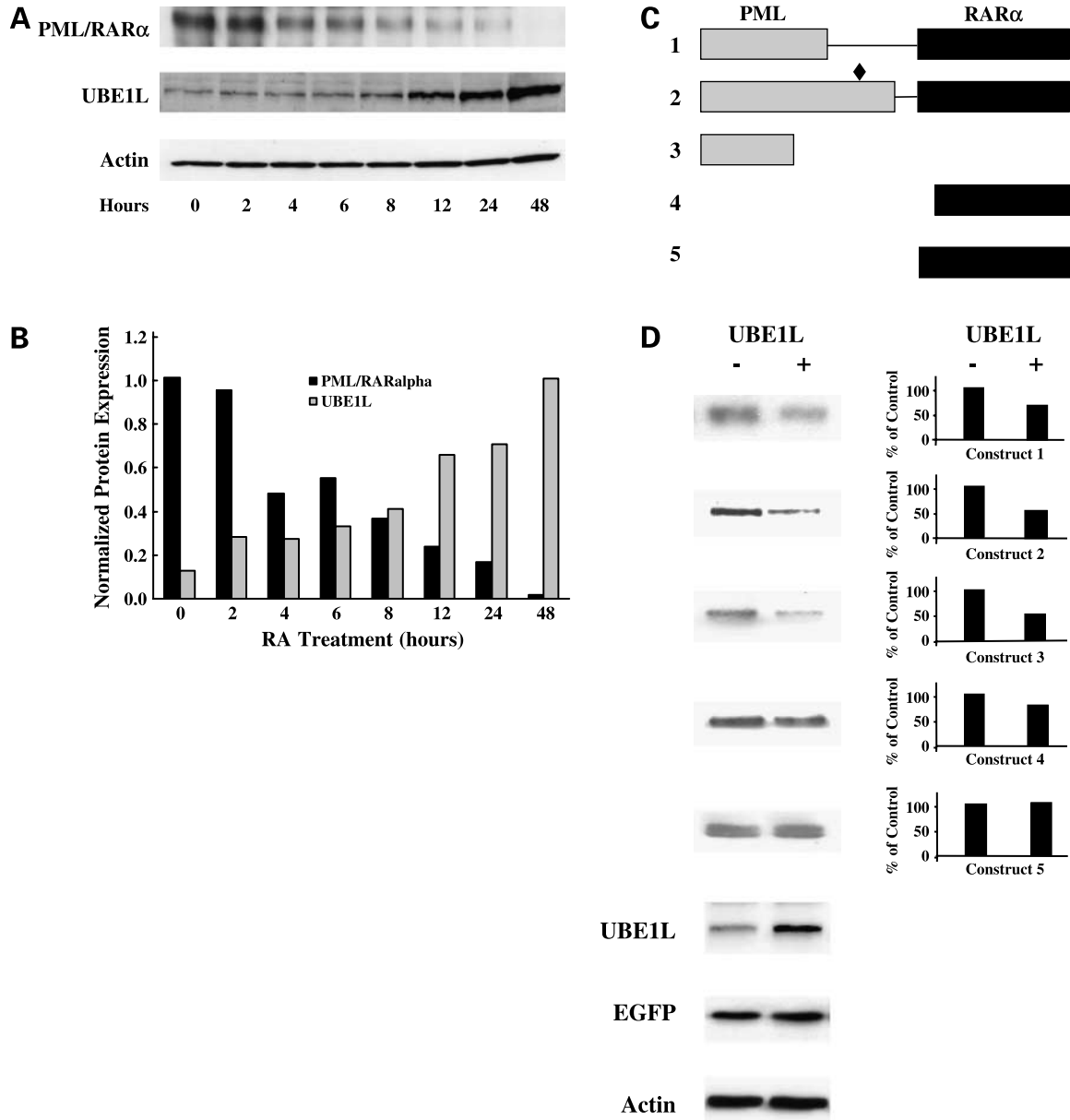
Figure 1. Immunoblot analyses of whole-cell lysates of NB4-S1 APL cells following RA treatment. A , NB4-S1 ( 2 \times 10^6 ) cells per experimental group were treated with RA (1 \mu mol/L) for 0 to 48 h and immunoblot analyses were done to assess effects of RA treatment on expression of PML/RAR \alpha and UBE1L. B , scanning densitometric analyses were done for the immunoblots displayed in A . Expression of PML/RAR \alpha and UBE1L was each normalized for actin expression, which served as a loading control. This study confirmed induction of UBE1L concurrent with PML/RAR \alpha repression following RA treatment of NB4-S1 APL cells. That UBE1L targeted the PML domain of PML/RAR \alpha was shown. C , schematic representation of five different PML/RAR \alpha expression constructs designated 1 to 5. Gray box, PML domain; black box, RAR \alpha domain. Construct 1 depicted PML/RAR \alpha (S), which differs from the PML/RAR \alpha (L) depicted in construct 2 in that it does not contain the aspartate residue at position 522 (black diamond), the known caspase-3 cleavage site (16). Expression vectors were also engineered to independently contain a portion of the PML domain (construct 3), a portion of the RAR \alpha domain (construct 4), or the entire RAR \alpha domain (construct 5) of PML/RAR \alpha . D , immunoblot analyses for UBE1L and UBE1L-mediated repression of protein products of constructs 1 to 5. Each construct was cotransfected with the UBE1L expression plasmid (+) or with an insertless control vector (-) in BEAS-2B cells followed by immunoblot analyses. Cotransfection of the EGFP expression vector served as a transfection control. Actin expression confirmed similar amounts of protein lysates were loaded. Expression levels of transfected UBE1L are displayed as are the indicated quantified signals. This experiment revealed that UBE1L mediates PML/RAR \alpha repression by targeting the PML domain of PML/RAR \alpha . PML/RAR \alpha (L) construct 2, PML domain construct 3, and RAR \alpha domain construct 5 were used for subsequent experiments.
