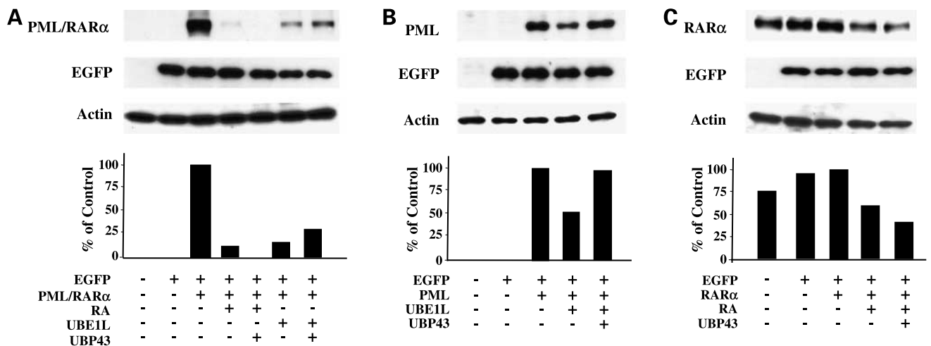
Figure 3. Independent effects of UBP43 on RA- and UBE1L-mediated repression of PML/RAR \alpha and its domains. BEAS-2B cells were independently transfected with (A) PML/RAR \alpha , (B) PML, or (C) RAR \alpha domain containing expression vectors. Indicated groups were either cotransfected with UBE1L or treated for 24 h with vehicle (DMSO) or RA (1 \mu mol/L). Cells were also cotransfected with or without a UBP43 expression vector as indicated. Immunoblot analyses revealed that UBP43 preferentially opposes UBE1L- but not RA-mediated repression of the indicated PML/RAR \alpha species. Bottom , quantification of each of these signals.
