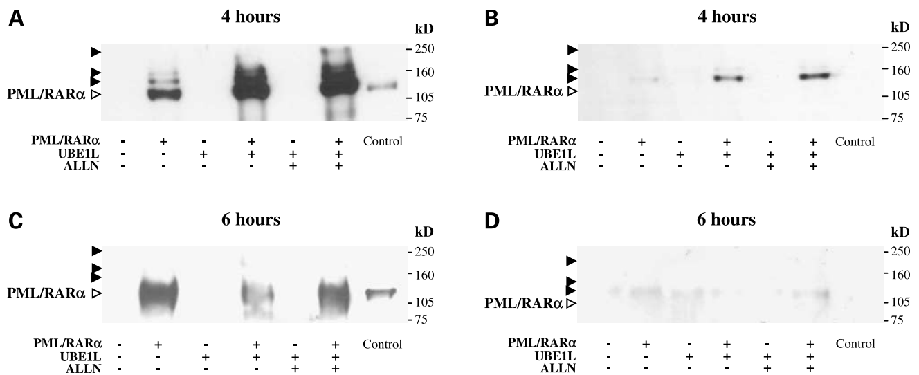
Figure 5. Effects of UBE1L on ISG15ylation of PML/RAR \alpha . BEAS-2B cells were individually transfected with PML/RAR \alpha containing expression constructs. Indicated groups were cotransfected with or without UBE1L. Following transfection, respective groups were treated with either ALLN (100 \mu M) or vehicle (DMSO) for 4 ( A and B ) or 6 ( C and D ) additional hours. Immunoprecipitation followed by immunoblot analyses were done as described in Materials and Methods. The filters were probed with either a monoclonal anti-HA antibody to detect PML/RAR \alpha ( A and C ) or a monoclonal anti-ISG15 antibody to detect ISG15ylated forms of PML/RAR \alpha ( B and D ). Open arrows , positions of unconjugated PML/RAR \alpha proteins; closed arrows , positions of post-translational modification products of PML/RAR \alpha ; Control , whole-cell lysates of COS-1 cells transfected with PML/RAR \alpha serve as a signal for unconjugated PML/RAR \alpha protein. These experiments established that UBE1L confers ISG15 conjugation to PML/RAR \alpha with subsequent repression of this protein.
