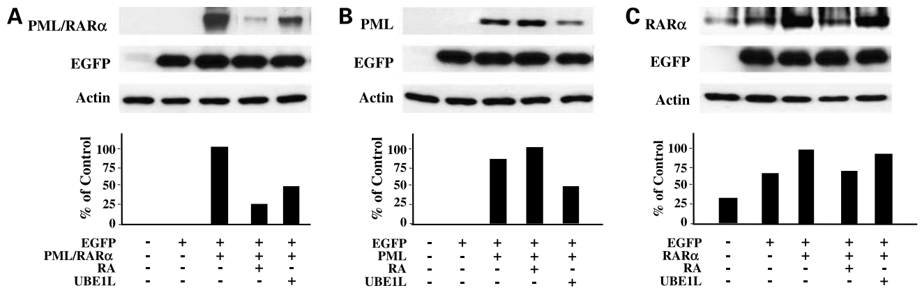
Figure 2. RA and UBE1L affect different PML/RAR \alpha domains. BEAS-2B cells were independently transfected with (A) PML/RAR \alpha , (B) PML, or (C) RAR \alpha expression constructs as described in Materials and Methods. Indicated groups were cotransfected with or without UBE1L and then treated for 24 additional hours with or without RA (1 \mu mol/L). Immunoblot analyses identified different domains of PML/RAR \alpha as being individually targeted by RA and UBE1L for repression of PML/RAR \alpha . Bottom , quantification of each of these signals.
