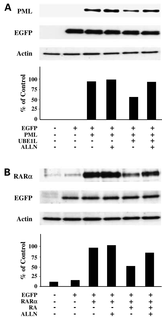
Figure 4. Effects of proteasome inhibition by ALLN on RA- and UBE1L-mediated repression of PML/RAR \alpha domains, respectively. BEAS-2B cells were independently transfected with (A) PML or (B) RAR \alpha domain containing expression constructs. Indicated groups were also cotransfected with or without UBE1L. Following transfection, cells in the ALLN treatment groups were incubated with ALLN (100 \mu mol/L) for 90 additional minutes. RA (1 \mu mol/L) was then added to the respective RA treatment groups and incubated for 6 additional h. Remaining groups were incubated with the vehicle (DMSO) during this same treatment period. Immunoblot analyses revealed that ALLN inhibited RA-dependent repression of the RAR \alpha domain and UBE1L-dependent repression of the PML domain of PML/RAR \alpha . Bottom , quantification of each of these signals.
