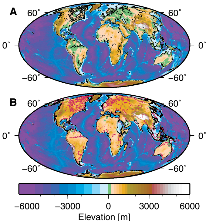
Figure 1. A: Earth's topography (Amante and Eakins, 2009; including ice, here plotted as land). B: What Earth might look like in the absence of mantle flow (see text for details). Actual coastlines are shown in black in A, and in maroon in B, and hypothetical coastlines are shown in black in B.
