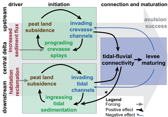
Figure 3. Progression of human-induced feedback mechanisms that lead to avulsion in compaction-prone deltas. Initially, human factors affected separate systems in areas upstream and downstream of peatlands, represented by two green boxes, which connect in central delta (blue box). Text in the boxes indicates processes; arrows indicate feedbacks. For explanation of asterisk, see main text.
