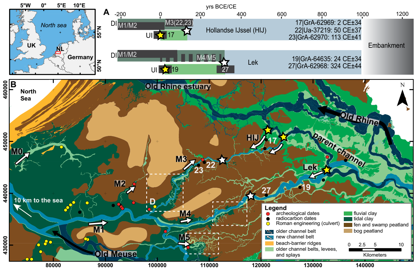
Figure 1. A: Time line of stage development of Hollandse IJssel (HIJ) and Lek avulsions, highlighting initiation phases at downstream (DI) and upstream (UI) locations. Main supporting ^{14}\text{C} dates ( \pm 1\sigma ) for samples from top of peat below river clay are indicated with black bars. M0–M5 indicate different tidal creeks from Old Meuse estuary; white rectangles indicate occurrence of rectangular creek networks. White stars indicate presumed tidal-fluvial connection moments and locations based on orientation and intersection of adjacent crevasse splays. Yellow stars indicate UI crevasse-avulsion initiation and position. B: Surficial geological map of study area showing old river courses (dark blue) and new courses (light blue; Cohen et al., 2012), flood-basin extent (green), and raised peat bogs (light brown; Van Dinter et al., 2014). Anthropogenic features of youngest 1000 yr were removed from map. Selected dates, relevant archaeological sites mentioned in text, and inferred stages of avulsion are indicated. See Data Repository (text footnote 1) for a full description of age control. UK—United Kingdom; NL—Netherlands. Map in RD projection, EPSG: 28992.
