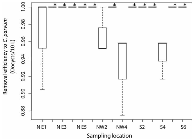
Figure 6 | Removal of Cryptosporidium parvum oocysts spiked in drinking water samples (10 L) processed by the multi-barrier device. The boxes show the variability between replicates and dashed lines the data distribution. *Oocyst removal for these samples was below the method limit of detection.
