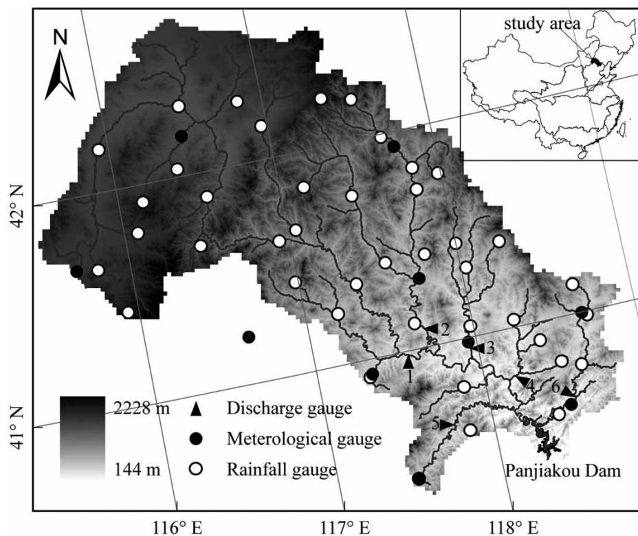
Figure 1 | Location of the study area in China and locations of discharge gauges, meteorological gauges and precipitation gauges (discharge gauges 1–6 are the Sandaohezi, Hanjiaying, Chengde, Xiabancheng, Liying, and Kuancheng, respectively).
