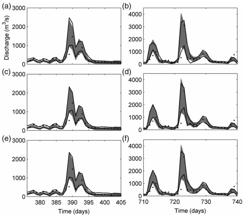
Figure 5 | Same as Figure 4, but for the Bagmati catchment.
