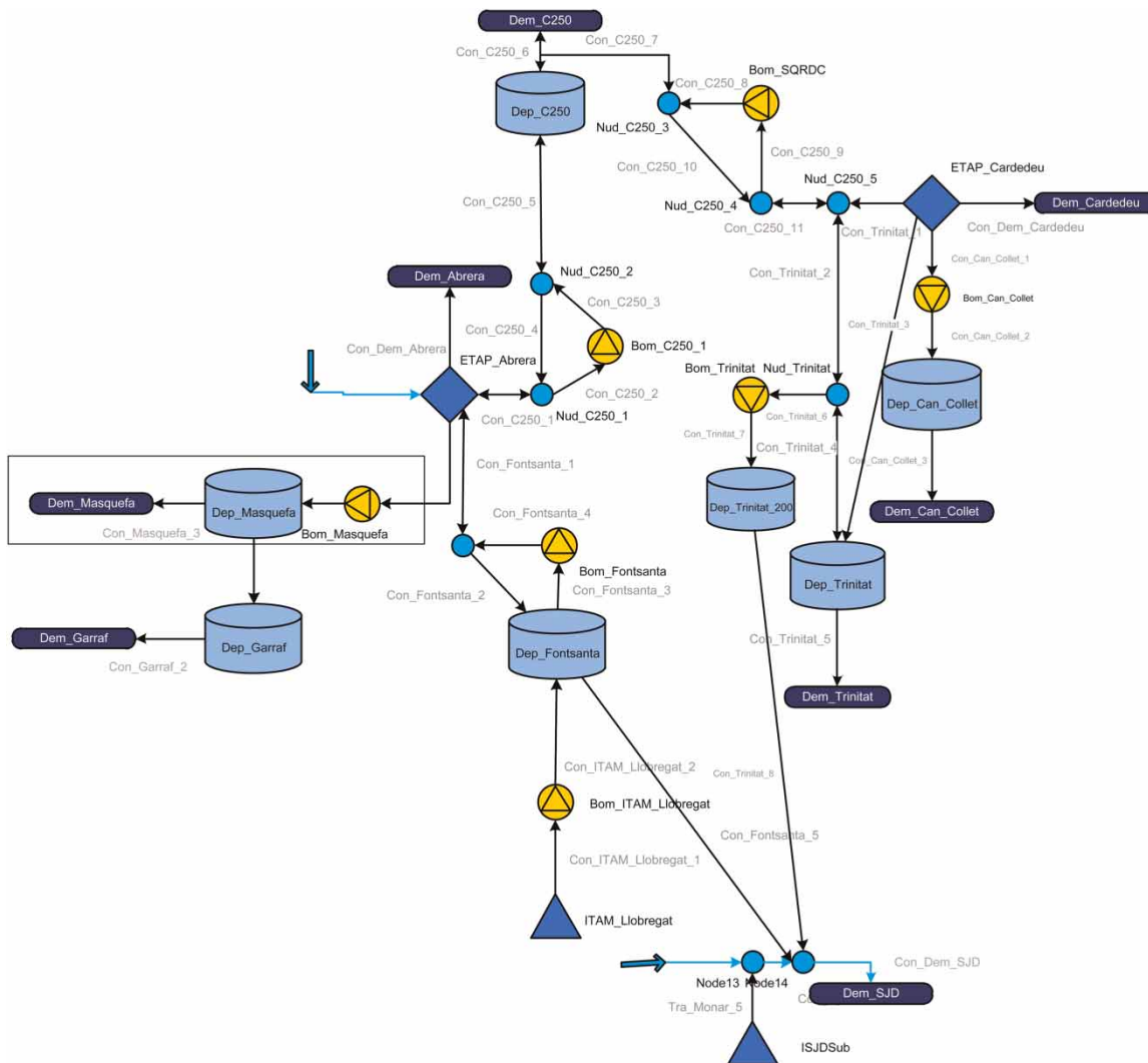
Figure 7 | Transportation network.
