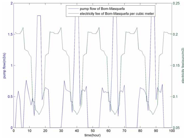
Figure 8 | Pump flow with electricity price.
