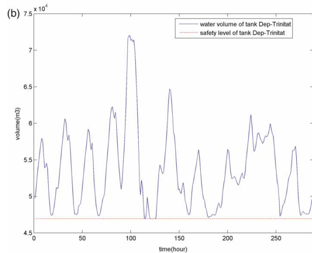
Figure 10 | Water level of tank Dep T rinitat before and after safety control starts from the date of 01/08/2011.
