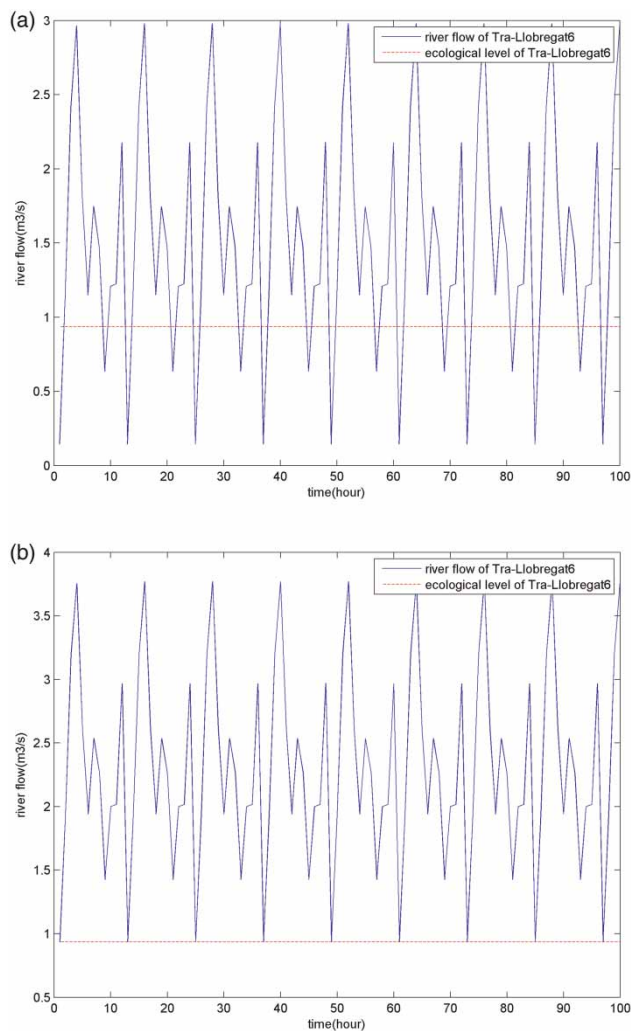
Figure 6 | River flow comparing ecological level (a) before and (b) after ecological control in River Llobregat.
