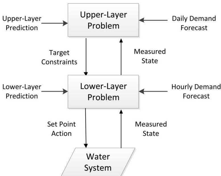
Figure 1 | Temporal hierarchy multi-layer MPC.
