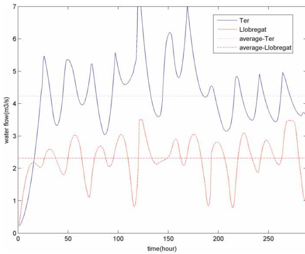
Figure 12 | Flows from the two rivers after using temporal coordination with x-time and y-flow axis.
