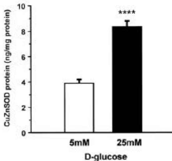
FIG. 6. CuZnSOD protein concentration (ng/mg protein) measured by ELISA in VSMCs cultured in 5 and 25 mmol/l D-glucose for 10 days. n = 15 independent experiments, each measured in duplicate. **** P < 0.00001 .
