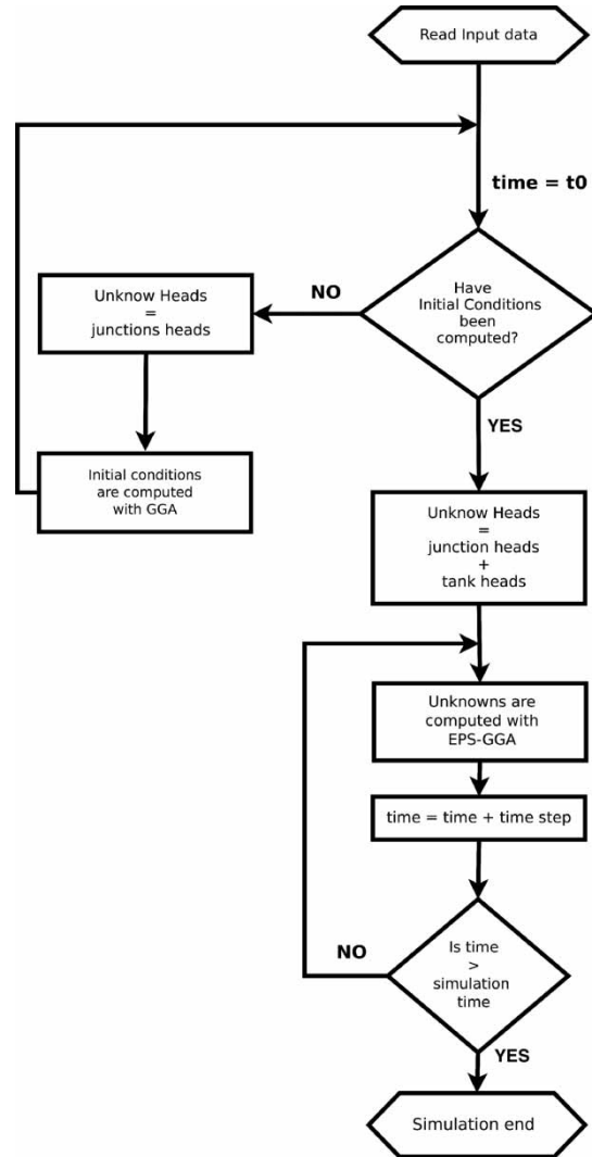
Figure 1 | EPS-GGA flowchart for the new code EPANET-EPS.
