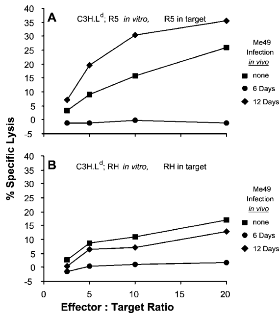
FIGURE 4. Kinetics and strain specificity of CTL following peroral infection with the Me49 strain of T. gondii . Specific lysis by C3H.L d effector cells is elicited by organisms of the R5 (A), but not the RH (B), strain of T. gondii at 12 days following infection, but by neither the R5 nor the RH strain of T. gondii at 6 days following infection. Splenocytes were harvested from uninfected C3H.L d mice (■) and from mice infected with cysts of the Me49 strain of T. gondii 6 days (●) or 12 days (◆) earlier and stimulated for 7 days in culture with either R5 (A) or RH (B) strain-irradiated T. gondii . Effector cells were not purified using Ficoll-Hypaque gradients or T cell enrichment columns. Effector cells were tested against uninfected P815 (H-2 d ; data not shown; the percent lysis at all E:T ratios was <10%) target cells or target cells infected with either R5 (A) or RH (B) strain T. gondii . Spontaneous lysis of targets was 24% or less. RH-infected target cells were 80% infected, and R5-infected target cells were 60% infected.
