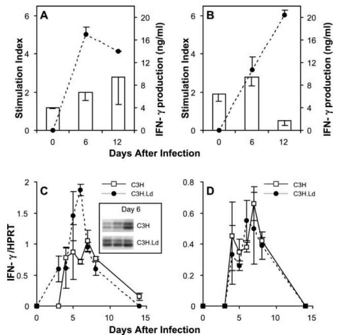
FIGURE 5. Lymphocyte proliferation, IFN- \gamma production, and mRNA expression following peroral T. gondii infection with the Me49 strain of T. gondii . A and B, TLA-induced proliferation of splenocytes (bars) and IFN- \gamma production (dotted line) in cultures from C3H.L d (A) or C3H/HeJ (B) mice. Splenocytes were isolated from uninfected mice and from mice 6 and 12 days following infection with cysts of the Me49 strain T. gondii . Spontaneous IFN- \gamma production from infected mice was below the detectable level on day 12, but in some cases was detectable, but <1 ng/ml on day 6. IFN- \gamma mRNA production was greater and occurred earlier in C3H.L d mice than in C3H/HeJ mice (C and D). Expt. C and D represent independent experiments. Three C3H.L d (●) and three C3H/HeJ (□) mice for each time point were infected perorally with 100 Me49 T. gondii cysts. On days 0, 3, 4, 5, 6, 7, 8, and 14 postinfection, their spleens were removed, and RT-PCR was performed on RNA from each mouse. IFN- \gamma message levels were semiquantitated as described in Materials and Methods , and the mean and SE were calculated. The inset in C shows the gels on day 6 in this experiment. The upper band is the competitor. Where the lower band is more prominent than the upper band, there is more competition by more IFN- \gamma in the sample. All PCR was performed within the linear range of amplification.
