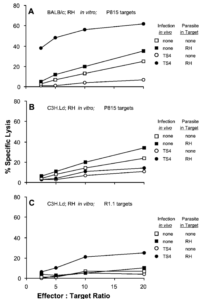
FIGURE 3. Genetic restriction and strain specificity of CTL following ts-4 immunization. Immunization with the ts-4 strain of T. gondii elicits CTL production in H-2 d mice that are not L d restricted. Splenocytes were harvested from nonimmunized (□ and ■) and ts-4-immunized (○ and ●) BALB/c ( A ) and C3H.L d ( B and C ) mice and were stimulated for 6 days in vitro with UV-attenuated RH strain T. gondii . Effector cells were tested against uninfected (○ and □) and RH-infected (● and ■) P815 (H-2 d ) or R1.1 (H-2 k ) target cells. Spontaneous lysis of target cells was 14% or less. Target cells were 50–55% infected.
