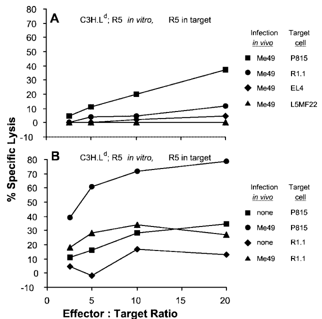
FIGURE 1. Genetic restriction and comparison of effector CTL from uninfected and infected C3H.L d mice. A , L d -restricted CTLs in spleens of T. gondii -infected C3H.L d mice. Splenocytes were harvested from C3H.L d mice infected with cysts of the Me49 strain of T. gondii 12 days earlier and stimulated in vitro for 7 days with UV-attenuated organisms of the R5 strain of T. gondii . Effectors were tested against uninfected (data not shown) or R5-infected (■, ●, ▲, and ◆) target cells. Target cells were P815 (H-2 d ; ■), R1.1 (H-2 k ; ●), EL4 (H-2 b ; ◆), and L5 MF22 (H-2 b ; ▲). Spontaneous lysis of target cells was 20% or lower for all target cells, with the exception of 30% for infected R1.1 cells. The percentages of infected cells were: P815, 70%; R1.1, 76%; EL4, 48%; and L5 MF22, 90%. All cultures with uninfected targets had <5% lysis at all E:T cell ratios (data not shown). B , Specific lysis of infected target cells by C3H.L d splenocyte effectors. Splenocytes were harvested from uninfected C3H.L d mice (■ and ◆) or C3H.L d mice 12 days following infection with Me49 strain of T. gondii (● and ▲) and were stimulated for 6 days in vitro with organisms of the R5 strain T. gondii attenuated with gamma irradiation. Effectors were tested against uninfected (data not shown) and R5-infected (■, ●, ▲, and ◆) P815 (H-2 d ; ■ and ●) and R1.1 (H-2 k ; ◆ and ▲) target cells. Spontaneous lysis of target cells was 16% or less for all target cells, with the exception of 42% for infected R1.1 cells. Seventy to 87% of target cells were infected. All cultures with uninfected targets had <10% lysis at all E:T cell ratios.
