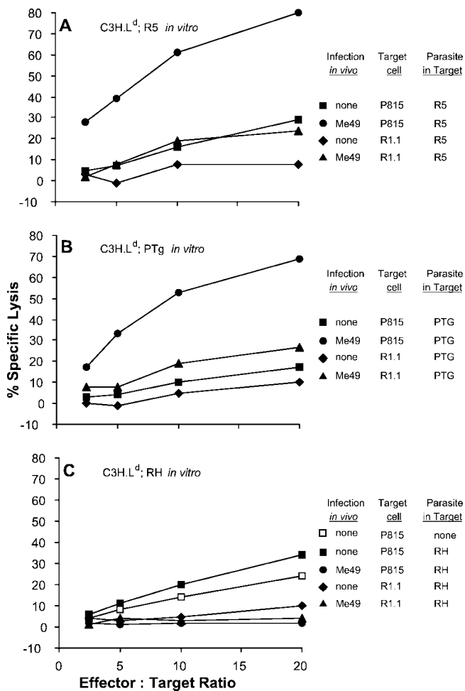
FIGURE 2. Splenocytes from T. gondii -infected C3H.L d mice exhibit L d specific lysis when cultured in vitro with either of two type II strains, but not a type I strain of T. gondii . A and B , Splenocytes were harvested from uninfected C3H.L d mice or from mice infected 12 days earlier with cysts of the Me49 strain T. gondii and stimulated for 6 days in vitro with R5 ( A ) or PTg ( B ) organisms attenuated by gamma irradiation. Effectors were tested against uninfected targets (data not shown, as lysis was <10% at all E:T cell ratios) and against R5 strain ( A ) and PTg strain ( B ) T. gondii -infected P815 (H-2 d ) and R1.1 (H-2 k ) target cells. Spontaneous lysis of all target cells was 23% or less, with the exception of 40% for R5-infected R1.1 target cells. R1.1 target cells were 38–55% infected. P815 target cells were 65% infected. C , Splenocytes were harvested as in described in A and B from mice infected 11 days and stimulated with the UV-attenuated RH strain T. gondii . Effectors were tested against uninfected (□; data not shown when lysis was <10% at all E:T cell ratios) and RH-infected (■) P815 and R1.1 target cells. Spontaneous lysis of targets was 14% or less for all target cells. Target cells were 50–55% infected.
