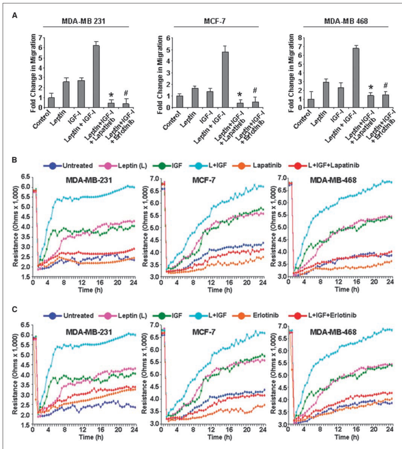
Figure 6. Inhibition of EGFR with lapatinib and erlotinib inhibits leptin- and IGF-I-induced increased migration of breast cancer cells. A , MDA-MB-231, MCF-7, and MDA-MB-468 breast cancer cells were grown to confluence on fibronectin-coated surface, serum starved for 24 h, and scratched with a pipette tip. The plates were photographed immediately following scratching. Culture media were replaced with media containing 100 ng/mL leptin, 100 ng/mL IGF-I alone, leptin + IGF-I, leptin + IGF-I + 2.5 \mu mol/L lapatinib, and leptin + IGF-I + 2.5 \mu mol/L erlotinib for 24 h. The plates were photographed at the identical location of the initial image at 24 h posttreatment. The fold change in migration was calculated. Columns, mean of three independent experiments done in triplicates; bars, SE. *, P < 0.005 , compared with leptin + IGF-I-treated cells; #, P < 0.001 , compared with leptin + IGF-I-treated cells. B and C , MDA-MB-231, MCF-7, and MDA-MB-468 cells were grown to confluence in ECIS plates, serum starved for 16 h, and subjected to an elevated voltage pulse of 40-kHz frequency at 3.5-V amplitude for 30 s to incite a wound. The cells were immediately treated with 100 ng/mL leptin, 100 ng/mL IGF-I alone, leptin + IGF-I, leptin + IGF-I + 2.5 \mu mol/L lapatinib, and leptin + IGF-I + 2.5 \mu mol/L erlotinib. The wound was then allowed to be healed by cells surrounding the small active electrode that did not undergo the elevated voltage pulse. Resistance was measured before and after the elevated voltage pulse application as described in Materials and Methods. The measurements were stopped 24 h after the creation of wound. All the experiments were done thrice in triplicates.
