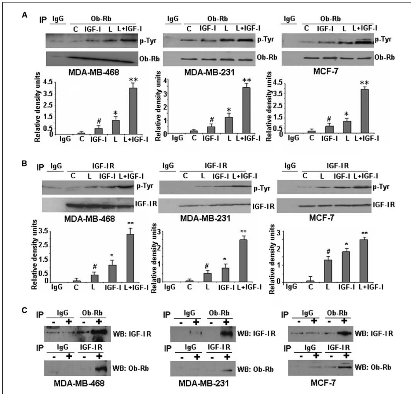
Figure 2. Evidence of crosstalk between leptin receptor (Ob-Rb) and IGF-IR. Leptin and IGF-I act synergistically to increase phosphorylation of Ob-Rb (A) and IGF-IR (B) in MDA-MB-468, MDA-MB-231, and MCF-7 breast cancer cells. Cells were serum starved for 24 h, followed by treatment with 100 ng/mL leptin (L), 100 ng/mL IGF-I alone (IGF-I), and the combination (L + IGF-I) for 30 min. C, untreated controls. Total protein was isolated and equal amounts of proteins were subjected to immunoprecipitation with specific antibodies for leptin receptor (A) or IGF-IR (B). Immunoprecipitates were resolved by SDS-PAGE and subjected to immunoblot analysis with a mouse monoclonal antibody against phospho-tyrosine. Immunoprecipitation with IgG was included as control (IgG). Leptin and IGF-I treatment increased phosphorylation of Ob-Rb whereas combined treatment induced further increase in Ob-Rb phosphorylation (A). Increased phosphorylation of IGF-IR was observed in cells treated with leptin and IGF-I alone, whereas combined treatment induced a synergistic increase in IGF-IR phosphorylation (B). Phosphorylated tyrosine bands shown in all cases correspond to the expected size band (Ob-Rb and IGF-IR). The membranes were reblotted with Ob-Rb and IGF-IR antibodies as control. Representative blots of multiple independent experiments. The histogram is the densitometric analysis of the Western blot signals normalized to total Ob-Rb or IGF-IR. #, P < 0.05 , compared with untreated controls; *, P < 0.05 , compared with untreated controls; **, P < 0.01 , compared with leptin-treated cells. C, association of Ob-Rb and IGF-IR occurs in breast cancer cells. MDA-MB-468, MDA-MB-231, and MCF-7 cells were serum starved for 24 h, followed by no treatment (-) or combined treatment with 100 ng/mL leptin (L) and 100 ng/mL IGF-I for 30 min (+). Total protein was isolated and equal amounts of proteins were subjected to immunoprecipitation with specific antibodies for Ob-Rb. The immunoprecipitates were probed with anti-IGF-IR antibody. In a reverse experiment, equal amounts of proteins were immunoprecipitated with anti-IGF-IR antibody and immunoprecipitates were probed with anti-Ob-Rb antibody. Immunoprecipitation with IgG was included as control (IgG). Both Ob-Rb and IGF-IR were coimmunoprecipitated in the presence of IGF-I and leptin, indicating the association of Ob-Rb and IGF-IR.
