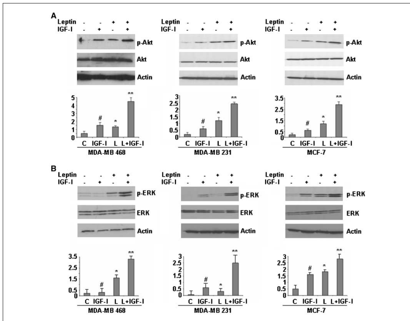
Figure 3. Combined treatment with leptin and IGF-I leads to a synergistic increase in phosphorylation of both Akt and ERK in breast cancer cells. MDA-MB-468, MDA-MB-231, and MCF-7 cells were serum starved for 24 h, followed by treatment with 100 ng/mL leptin, 100 ng/mL IGF-I alone, and the combination for 30 min. Total protein was isolated from MDA-MB-468, MDA-MB-231, and MCF-7 cells and equal amounts of proteins were subjected to immunoblot analysis with specific antibodies against phospho-Akt ( p-Akt ) and Akt (A) or phospho-ERK ( p-ERK ) and ERK (B). Increased phosphorylation of Akt was observed in MDA-MB-468, MDA-MB-231, and MCF-7 cells treated with leptin or IGF-I, whereas combined treatment induced further increase in Akt phosphorylation. Leptin and IGF-I treatment increased phosphorylation of ERK, whereas combined treatment induced a synergistic increase in ERK phosphorylation. The membranes were reblotted with ERK, Akt, and anti-actin antibodies as control. Representative blots of multiple independent experiments. The representative histogram is the densitometric analysis of the Western blot signals showing fold increase in levels of phospho-Akt and phospho-ERK with respect to total Akt and ERK. #, P < 0.01 , compared with untreated controls; *, P < 0.05 , compared with untreated controls; **, P < 0.01 , compared with leptin-treated cells.
