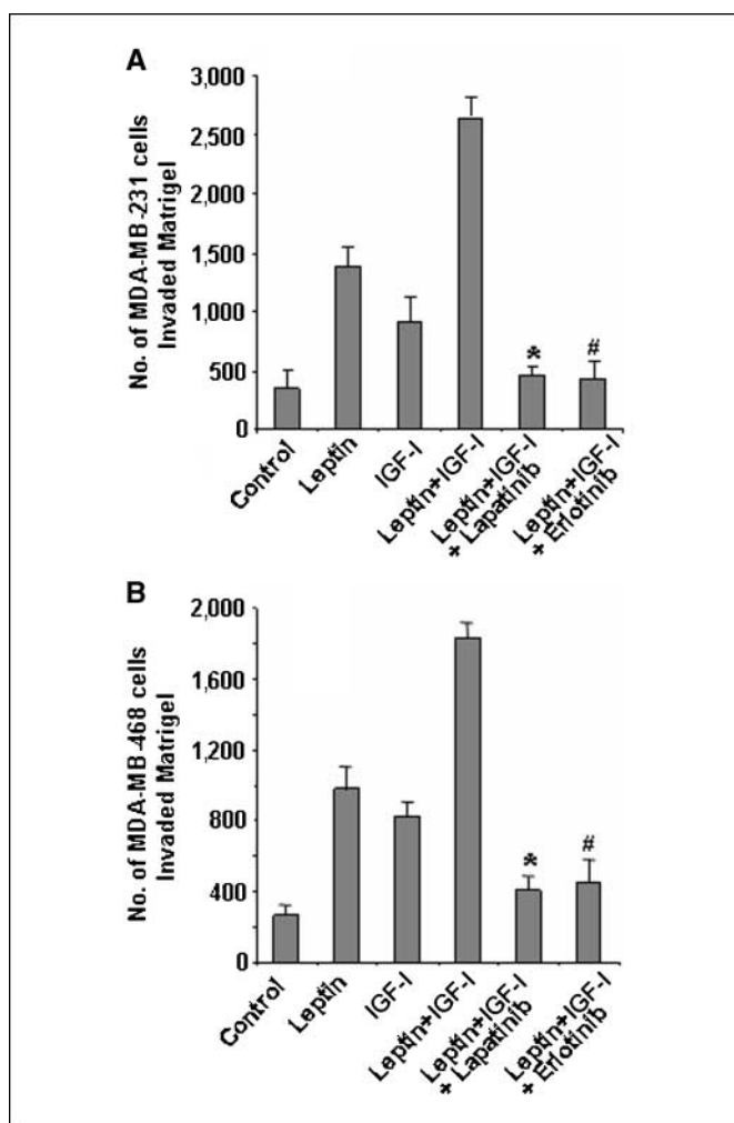
Figure 5. Lapatinib and erlotinib inhibit leptin- and IGF-I-induced increased invasion of breast cancer cells. MDA-MB-231 (A) and MDA-MB-468 (B) cells were cultured in Matrigel invasion chambers and serum starved for 24 h, followed by treatment with 100 ng/mL leptin, 100 ng/mL IGF-I alone, leptin + IGF-I, leptin + IGF-I + 2.5 \mu Mol/L lapatinib, and leptin + IGF-I + 2.5 \mu Mol/L erlotinib for 24 h. The number of cells that invaded through the Matrigel was counted in five different regions. The slides were blinded to remove counting bias. Columns, mean of three independent experiments done in triplicates; bars, SE. *, P < 0.001 , compared with leptin + IGF-I-treated cells. #, P < 0.001 , compared with leptin + IGF-I-treated cells.
