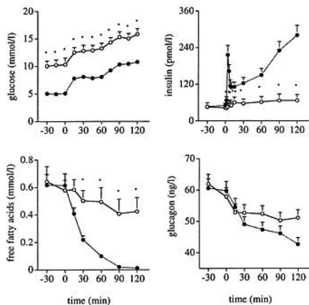
FIG. 1. Plasma glucose, insulin, free fatty acids, and glucagon concentrations during a two-step hyperglycemic clamp in MODY3 patients (○) and healthy subjects (●). * P < 0.05 vs. healthy subjects.
