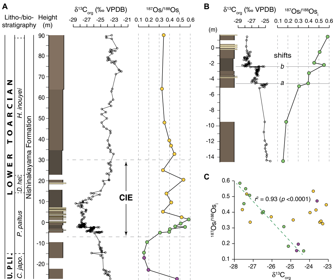
Figure 2. Os-isotope and organic \delta^{13}\text{C} ( \delta^{13}\text{C}_{\text{org}} ) through the Sakuraguchi-dani succession, Japan. (A) Sedimentary log with ^{187}\text{Os}/^{188}\text{Os}_i (i—initial) and \delta^{13}\text{C}_{\text{org}} variations against lithostratigraphy and ammonite zones ( C. japo. — Canavaria japonica ; P. paltus — Paltarpites paltus ; D. heli. — Dactylioceras helianthoides ; H. inouyei — Harpoceras inouyei ). Color-coding divides ^{187}\text{Os}/^{188}\text{Os}_i data into pre-carbon-isotope excursion (CIE) data (purple), data primarily through onset of the CIE (minimum to maximum ^{187}\text{Os}/^{188}\text{Os}_i , green), and data above these (orange). Log is from Izumi et al. (2012, 2018a) and field observations. \delta^{13}\text{C}_{\text{org}} is from Izumi et al. (2012, 2018a, 2018b), Kemp and Izumi (2014), and this study. PLI.—Pliensbachian; VPDB—Vienna Pee Dee belemnite. (B) Close-up of the CIE onset, showing abrupt shifts in ^{187}\text{Os}/^{188}\text{Os}_i across \delta^{13}\text{C}_{\text{org}} shifts a and b . (C) Crossplot of ^{187}\text{Os}/^{188}\text{Os}_i and \delta^{13}\text{C}_{\text{org}} showing the negative correlation between ^{187}\text{Os}/^{188}\text{Os}_i and \delta^{13}\text{C}_{\text{org}} across the onset of the CIE/ ^{187}\text{Os}/^{188}\text{Os}_i excursion, and no correlation below and above this interval.
