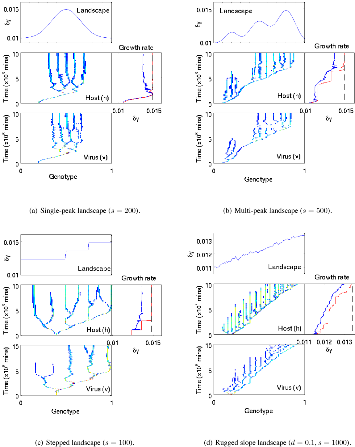
Figure 3: Case study simulations showing coevolutionary dynamics and host growth rate adaptation on various growth landscapes. Plots show the growth landscape ( top , given as the value of \delta_i\gamma for all possible host genotypes h_i ), the distribution over time of hosts and viruses in genetic space ( middle and bottom ), and the observed growth rates over time of the host community ( right , shows mean (blue), actual maximum (red), potential maximum (dashed)).
