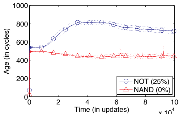
(b) Ancestor: NAND-NOT; Treatment: NOT is risky
