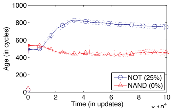
(a) Ancestor: NOT-NAND; Treatment: NOT is risky
