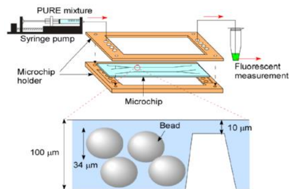
Fig. 1. Design of a microchip
