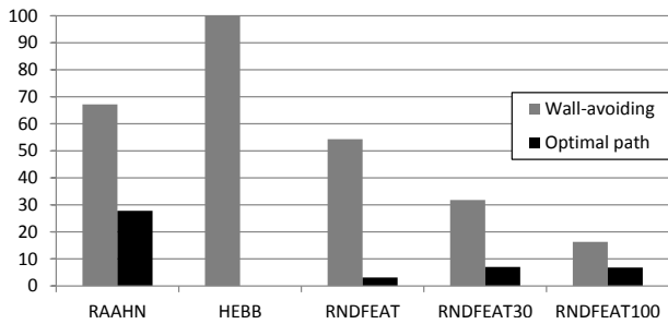
Figure 4: Percentage of wall-avoiding and optimal path followers. Results for each variant are percentages calculated over 1 000 evaluations.
