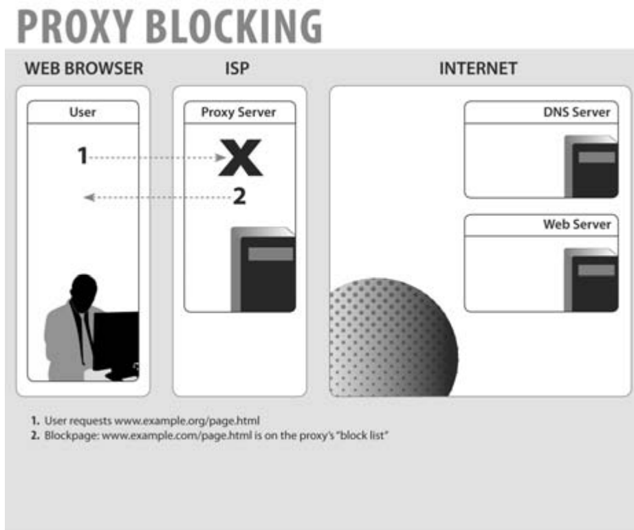
Figure 3.5 HTTP proxy blocking.
