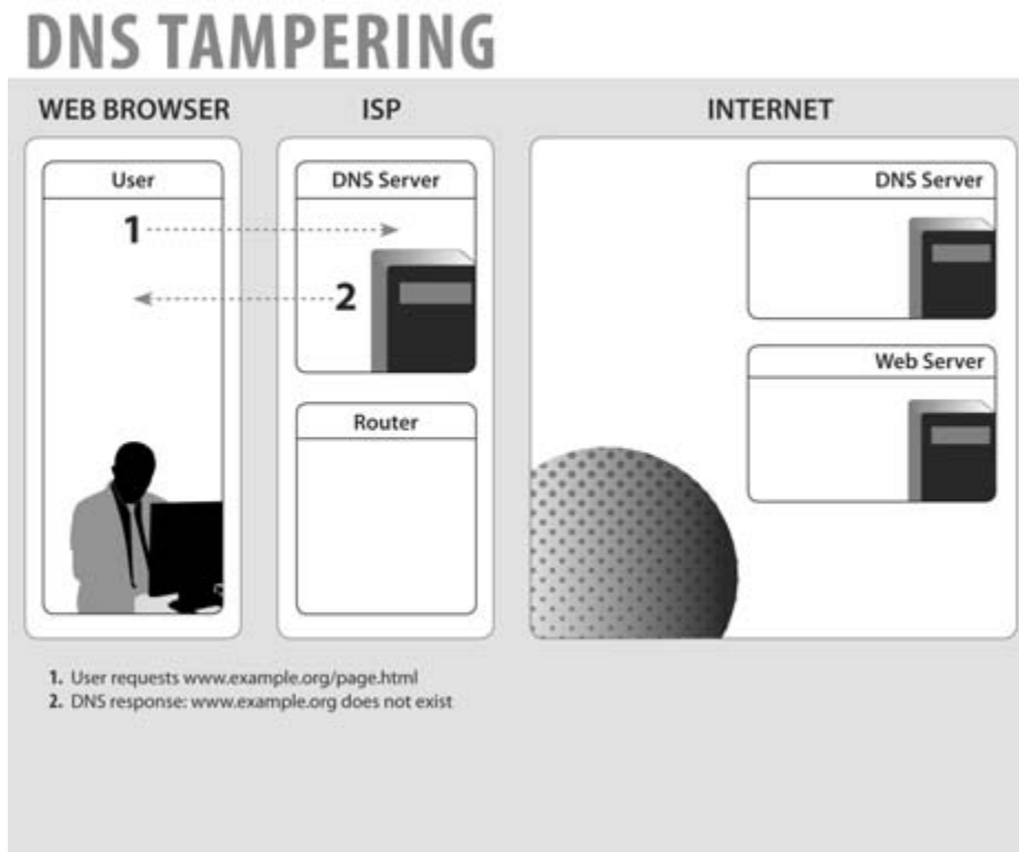
Figure 3.3 DNS tampering via filtering mechanism.
