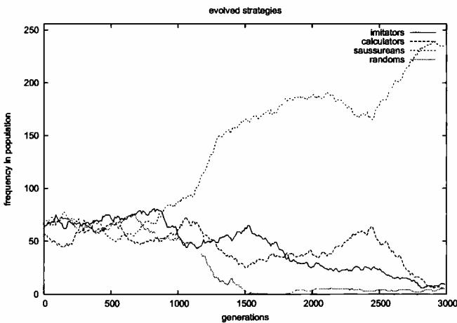
Figure 2: Evolved strategies
