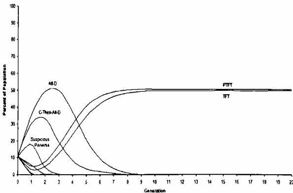
Figure 2. Percentages of the population for 9 strategies in an array segregated by color. 20 generations shown.
