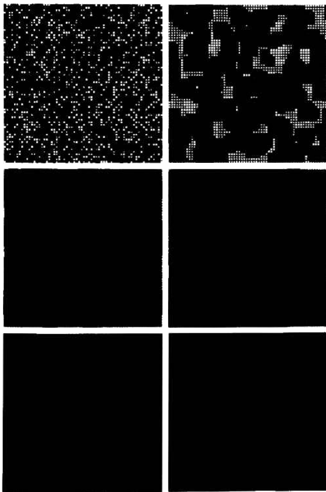
Figure 6. Evolution of randomized strategies to dominance by TFT (shown in black) in an integrated color array. Generations 0, 4, 8, 12, 16, and 20 shown.
