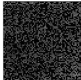
Figure 4. An integrated array of red and green (shown as shades of gray)
