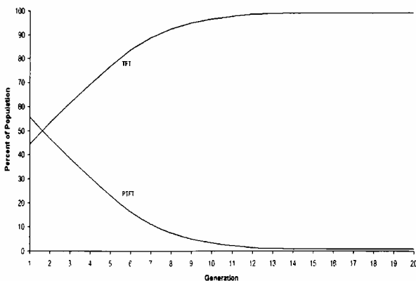
Figure 9. The Elimination of Established Prejudice: Triumph by TFT from scattered territories of PTFT and TFT in an array randomized by color.
