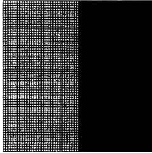
Figure 1. A segregated array of red and green (shown here as shades of gray)
