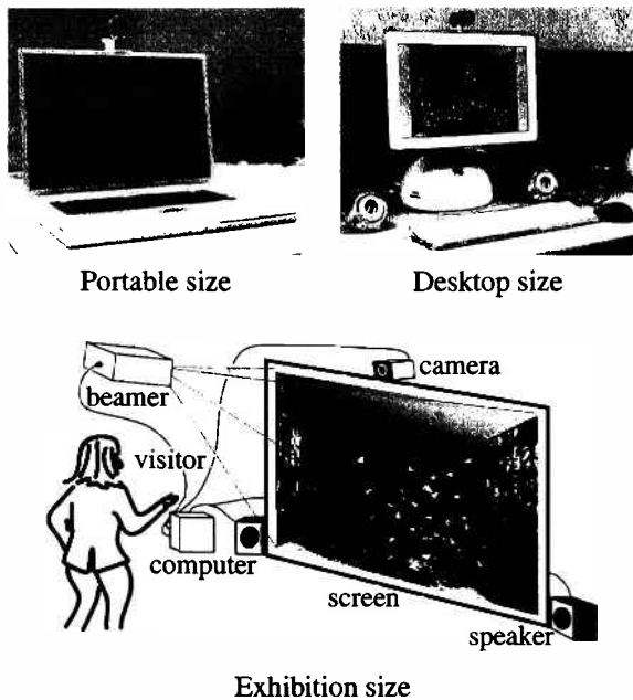
Figure 8: Typical system configurations in various sizes.
