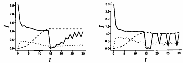
Figure 7: Information flows constructed by the best evolved 6-state (left) and 8-state (right) controller pairs. Solid line – I(M_0; M_t) , dashed – I(M_0; B_t) , dotted – I(R_0; M_t) .
