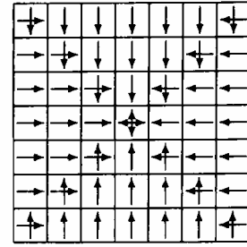
Figure 3: Sensoric input S vs. the position R . In cells with only one arrow the input is constant. In cells with multiple arrows it is randomly chosen from the listed options. The source is located at the center of the grid.
