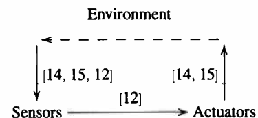
Figure 1: Information flow within an agent (box) and between the agent and its environment addressed by quantitative information-theoretic approaches. Solid line – prior work. Dashed and solid – this paper.
