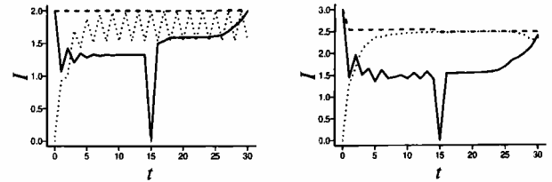
Figure 5: Information flows constructed by the best evolved 4-state (left) and 8-state (right) controller. Solid line – I(M_0; M_t) , dotted – I(M_0; R_t) , dashed – I(M_0; M_t, R_t) .
