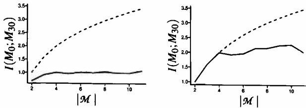
Figure 6: Fitness of best evolved controllers. Left: initial position of the sender is distributed over 11 \times 11 cells, Right: the sender always starts at the source. Dashed line – theoretical upper bound \log_2 |\mathcal{M}| .
