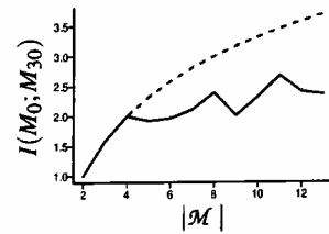
Figure 4: Fitness of best evolved controllers. Solid line – fitness measured as the information flow I(M_0; M_{30}) for controllers with |\mathcal{M}| states. Dashed line – theoretical upper bound \log_2 |\mathcal{M}| .
