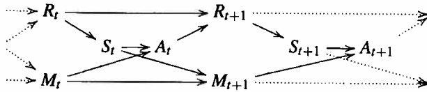
Figure 2: A temporal section of the unrolled perception-action loop modeled as a Bayesian network. The dotted lines show how the section connects to adjacent sections. S – sensoric input, A – action performed, M – memory of the controller, R – the rest of the world.
