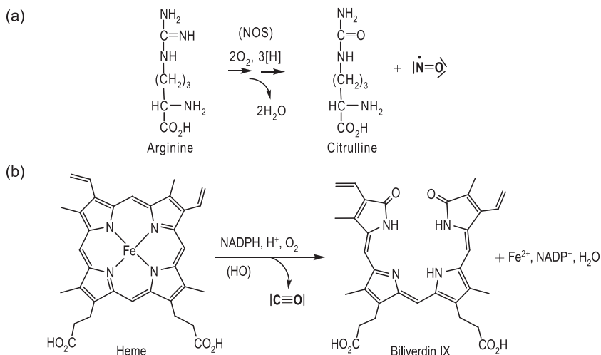
Figure 13.3 (a) Formation of nitric oxide: NO is catalyzed by nitrogen oxide synthase, NOS, in a two-step process via an [NOH] intermediate. [H] represents reduction equivalents, commonly delivered by nicotine adenine dinucleotide NADPH. (b) Carbon monoxide (CO) forms by oxidative catabolism of free heme, catalyzed by heme oxygenase (HO). A potent inducer for the transcription of the HO-1 gene is nitric oxide.
