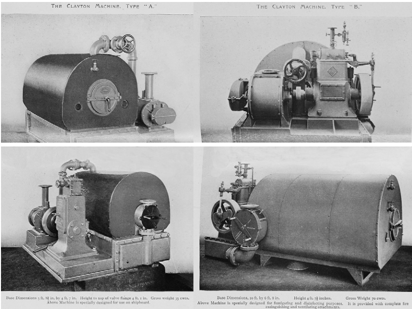
Figure 4.1 Two types of the Clayton machine from promotional pamphlet, “The Clayton Fire Extinguishing and Ventilating Company, Limited.” Credit: The National Archives (UK), ref. MH19/274.
