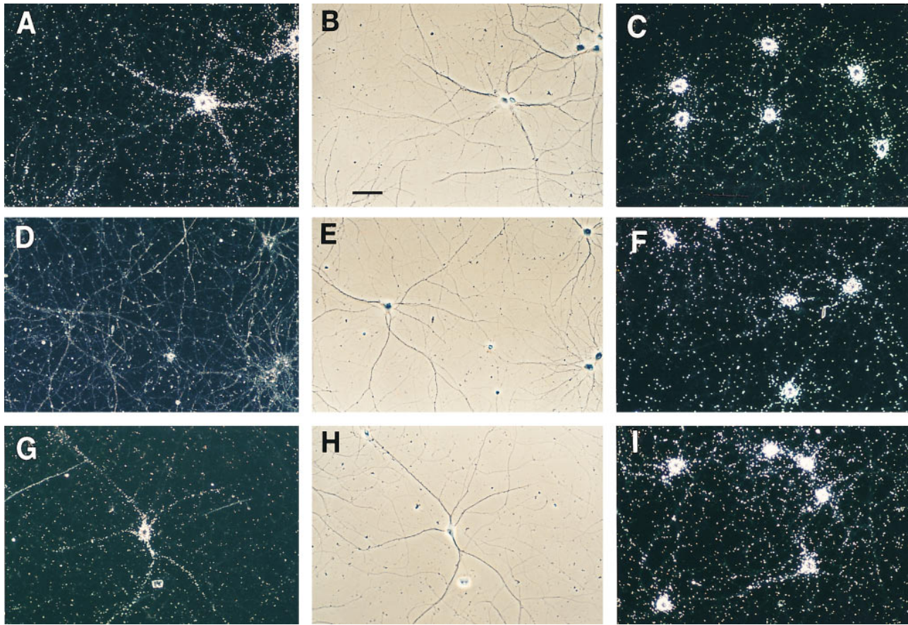
Figure 5. Regulation of BC1 expression by neuronal activity. Hippocampal neurons were grown in culture for 14 d in the absence of TTX (A–C), in the presence of 1 \mu M TTX (D–F), or in the presence of 1 \mu M TTX for the first 9 d, and in the absence of TTX for the following 5 d (G–I). Left (A–G): BC1 RNA, dark-field photomicrographs; middle (B–H), BC1 RNA, phase contrast photomicrographs, corresponding to dark-field photomicrographs in left column; right (C–I): 7SL RNA, dark-field photomicrographs. Dark field photomicrograph D (BC1 RNA in the presence of TTX) was overexposed to reveal absence of any significant labeling over cells or neurites. All cultures were grown at medium density. Bar, 50 \mu m. (J) Cultured hippocampal neurons
