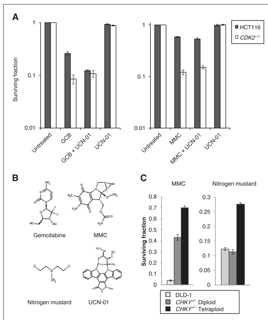
Figure 6. Effects of a Chk1 inhibitor and cell ploidy. A , wild-type HCT116 and CDK2 -/- cells were treated for 24 hours with 100 nmol/L UCN-01 alone or in combination with 20 nmol/L gemcitabine (GCB; left) or 150 nmol/L MMC (right). B , chemical structures of gemcitabine, MMC, UCN-01, and nitrogen mustard. C , CHK1 +/- cells that were primarily diploid were compared with wild-type DLD-1 and an isolated subclone of CHK1 +/- tetraploid cells. All cells were treated with the alkylating agents MMC (1 μmol/L) or nitrogen mustard (1 μmol/L) for 24 hours. Clonogenic survival is expressed as proportional survival compared with untreated controls of the same genotype.
