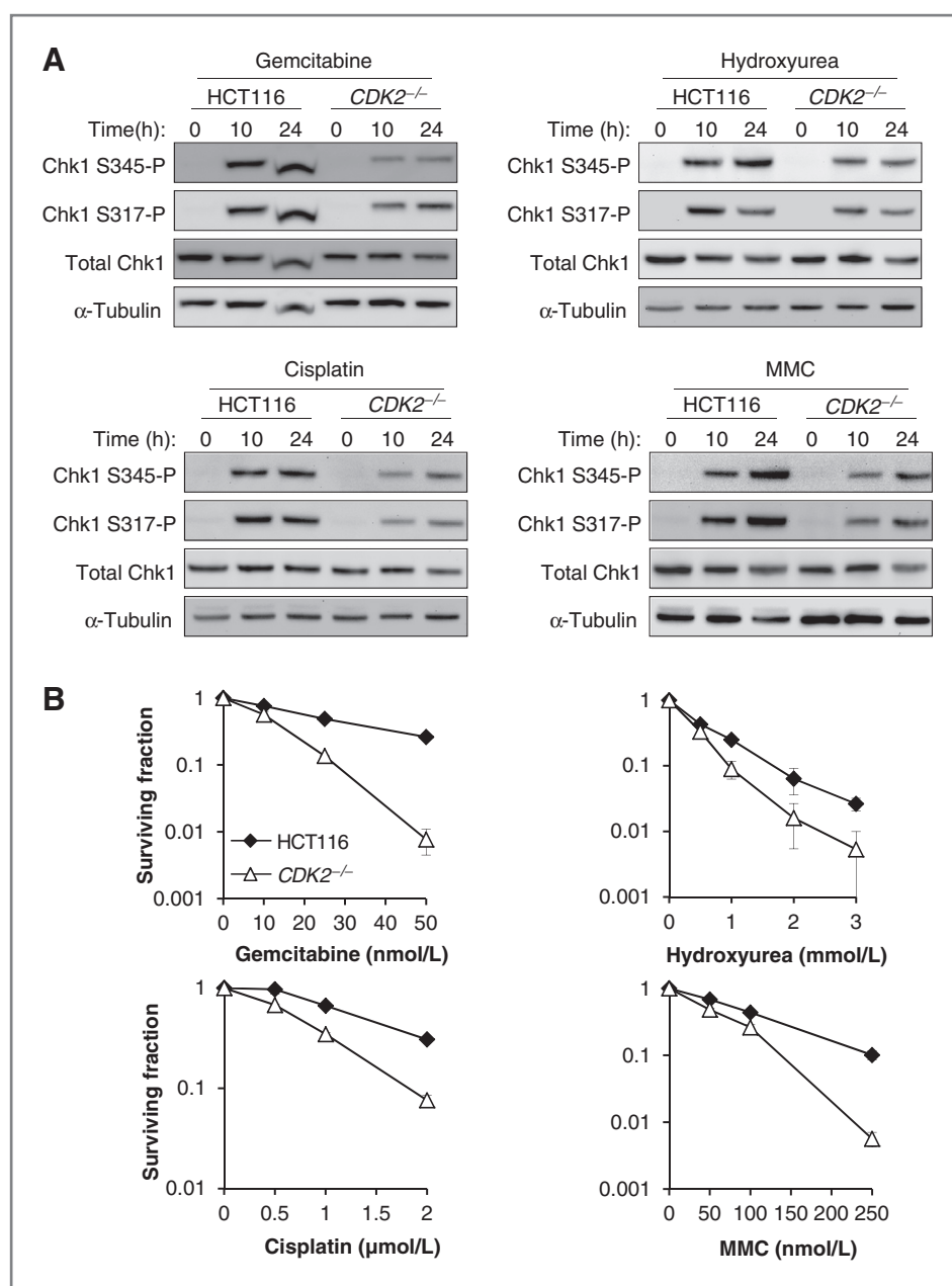
Figure 5. The role of Cdk2 in the cellular responses to ATR genotype-selective agents. A , HCT116 and isogenic CDK2 -/- cells were treated with the indicated chemotherapeutic agents and harvested at 10 or 24 hours. Time "0" indicates no treatment. Levels of the Chk1 phosphoproteins Chk1S345-P and Chk1S317-P and total Chk1 were determined by immunoblotting. \alpha -Tubulin was assessed as a loading control. B , clonogenic survival was measured in wild-type HCT116 and CDK2 -/- cells treated with gemcitabine, hydroxyurea, or MMC for 24 hours or cisplatin for 48 hours, as indicated.
