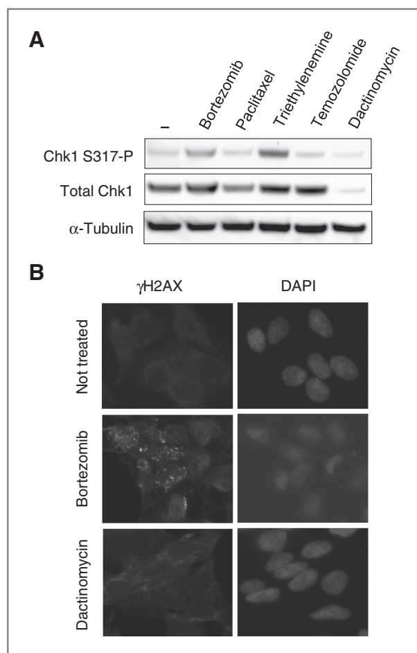
Figure 4. Phosphorylation of Chk1 in response to genotype-selective chemotherapeutics. A , levels of total Chk1 protein and Chk1 S317-P phosphoprotein in drug-treated DLD-1 cells were determined by immunoblotting. Drug concentrations used were bortezomib (300 nmol/L), paclitaxel (300 nmol/L), temozolomide (1 \mu mol/L), triethylenemelamine (1 \mu mol/L), and dactinomycin (300 nmol/L). Lysates were harvested after 24 hours of drug treatment. B , DLD-1 cells were treated with 300 nmol/L bortezomib or 300 nmol/L dactinomycin for 24 hours. The localization and distribution of \gamma H2AX were assessed by immunofluorescence. Nuclei were counterstained with 4',6-diamidino-2-phenylindole (DAPI).
