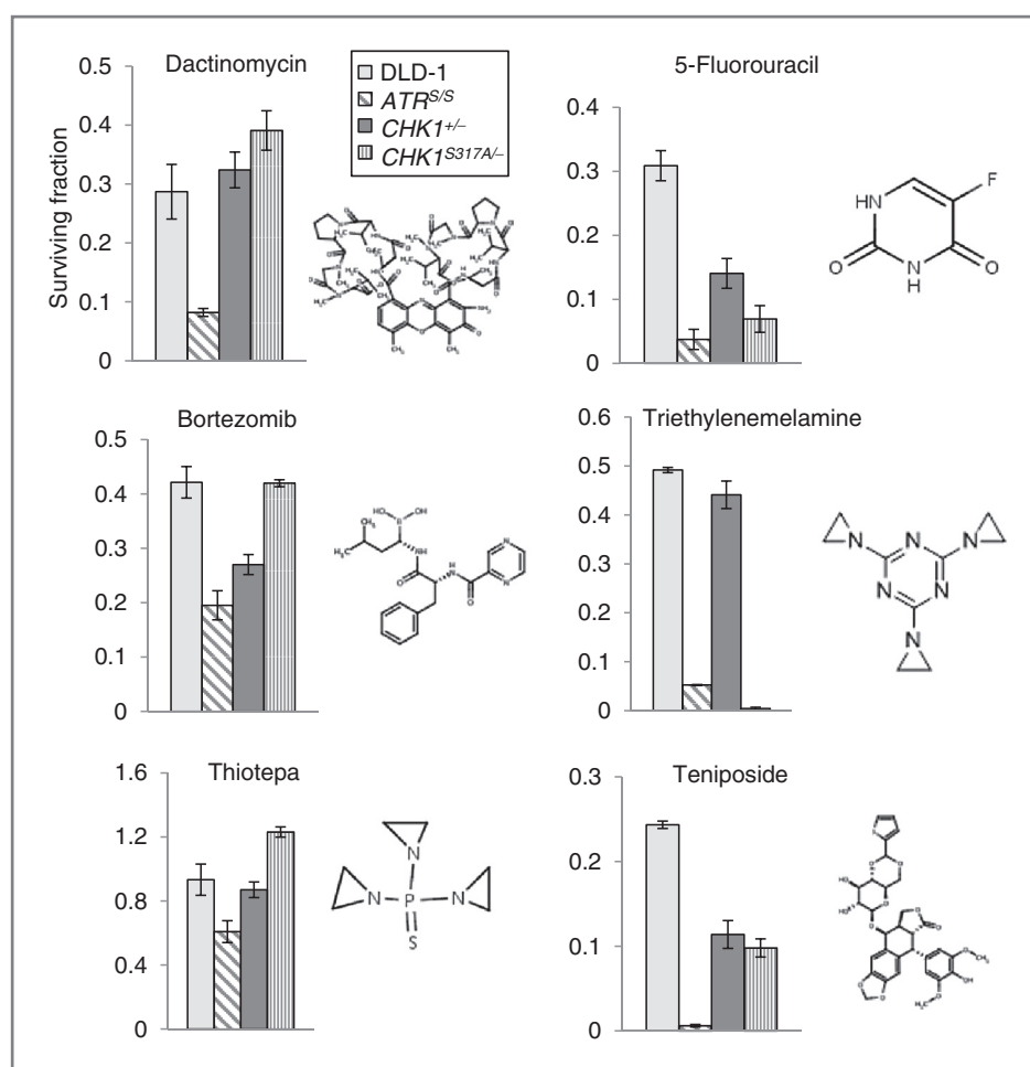
Figure 3. Inhibition of cell survival after treatment with selected anticancer agents. DLD-1 cells were compared with their isogenic derivatives in a clonogenic survival assay. Drug concentrations used were bortezomib (30 nmol/L), thiotepa (1 \mu mol/L), triethylenemelamine (1 \mu mol/L), dactinomycin (30 nmol/L), teniposide (300 nmol/L), and 5-fluorouracil (50 \mu mol/L). Cell lines were treated with drugs for 24 hours before replating.
