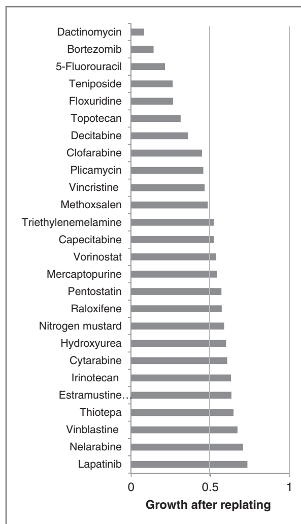
Figure 2. Inhibition of cell growth after treatment with anticancer agents. DLD-1 cells were compared with their ATR^{S/S} derivative in a high-throughput growth assay (see Materials and Methods). The growth of ATR^{S/S} cells was plotted as the proportional growth of wild-type DLD-1 cells treated with the same drugs.
