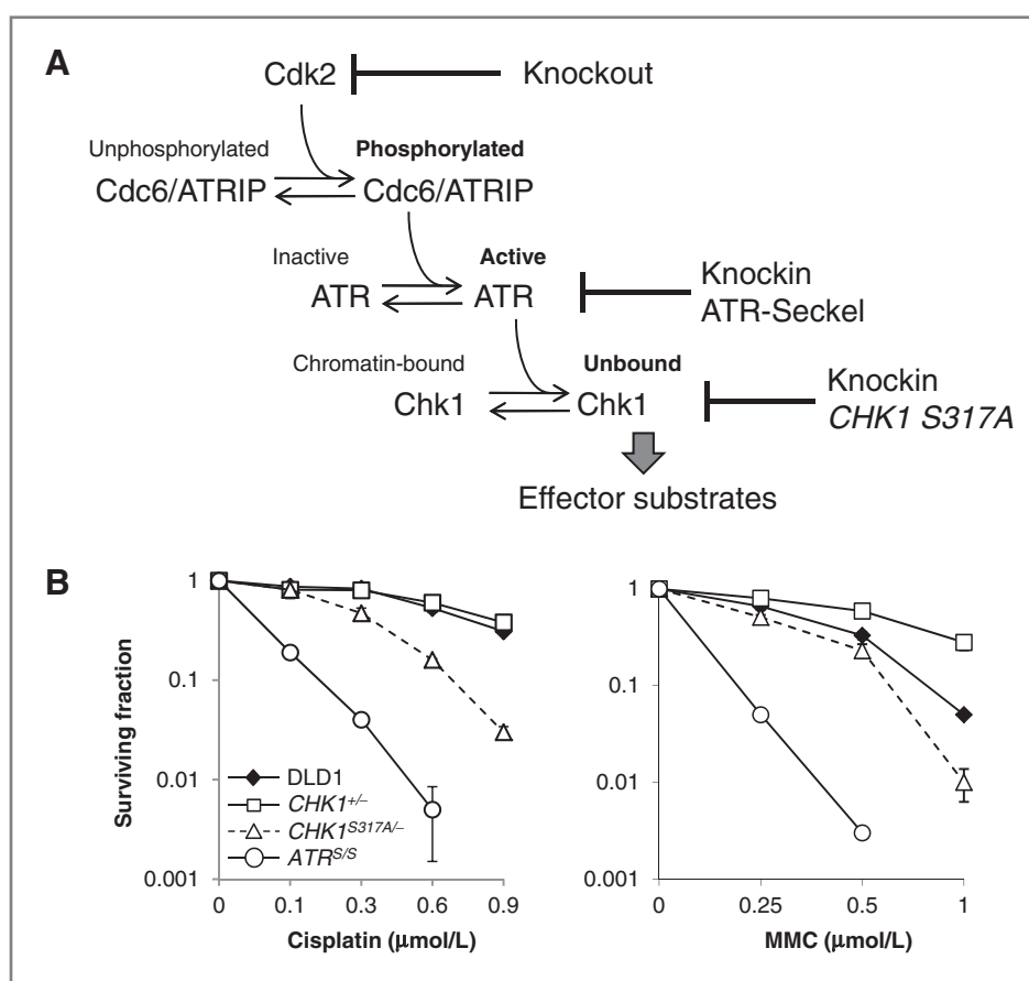
Figure 1. Evaluating drug responses in genetically modified human colorectal cancer cell lines. A , ATR can be activated during S-phase in the presence of upstream Cdk2. The contributions of individual components of the Cdk2/ATR/Chk1 pathway were assessed with the use of isogenic lines harboring knockout and knockin alleles, as indicated. See text for additional details. B , clonogenic survival of DLD-1 and ATR S/S , CHK1 +/- and CHK1 S317A/- derivative cells after treatment with the indicated doses of drugs. Survival is plotted on log scale as a proportion of untreated controls.
