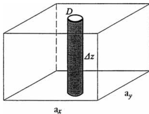
Figure 2 | Notation used in definition of vegetation density \lambda .
