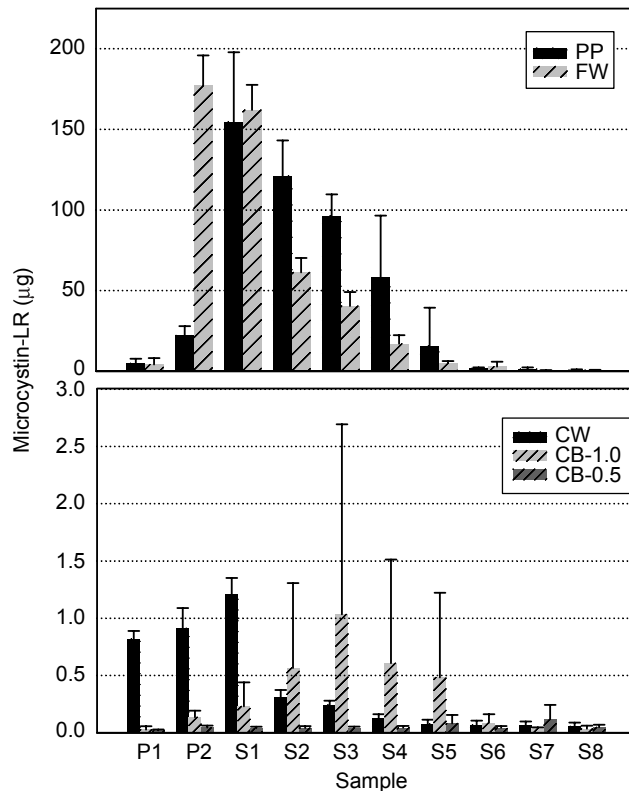
Figure 4 | Micrograms of microcystin recovered for the various filters studied vs. filter sequence number. (PP = pleated paper, FW = fibre wound, CW = carbon wrapped, CB-1.0 = carbon block 1 \mu\text{m} , CB-0.5 = carbon block 0.5 \mu\text{m} ).
