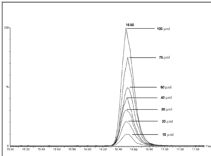
Figure 3 | Overlay of chromatographs obtained for a representative set of calibration injections ranging from 10 to 100 ng.
