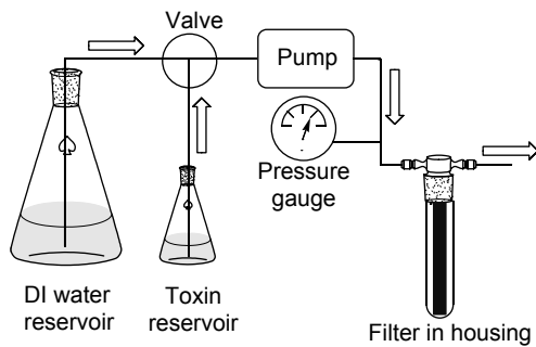
Figure 2 | Filtration apparatus.
