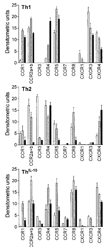
FIGURE 2. Densitometric analysis of chemokine receptor mRNAs expressed by resting and activated T cell clones. Densitometric values were calculated from RNase protection assay by laser densitometry and normalized against the housekeeping gene L32. Results are expressed as the mean \pm SD of experiments performed on four Th IL-10 , two Th1, and two Th2 clones. Open columns, resting T cells; hatched columns, 6-h activated T cells; and filled columns, 48-h activated T cells.
