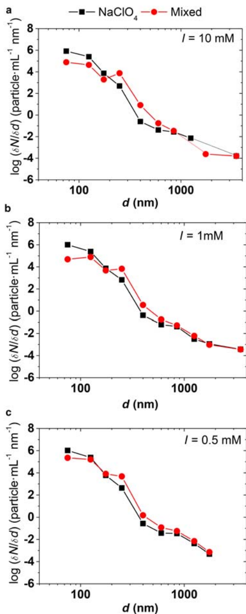
FIG. 5. Size distribution of suspensions in \text{NaCl-CaCl}_2 (●) and \text{NaClO}_4 (■) at different ionic strengths: (a) 10 mM; (b) 1 mM; and (c) 0.5 mM.
