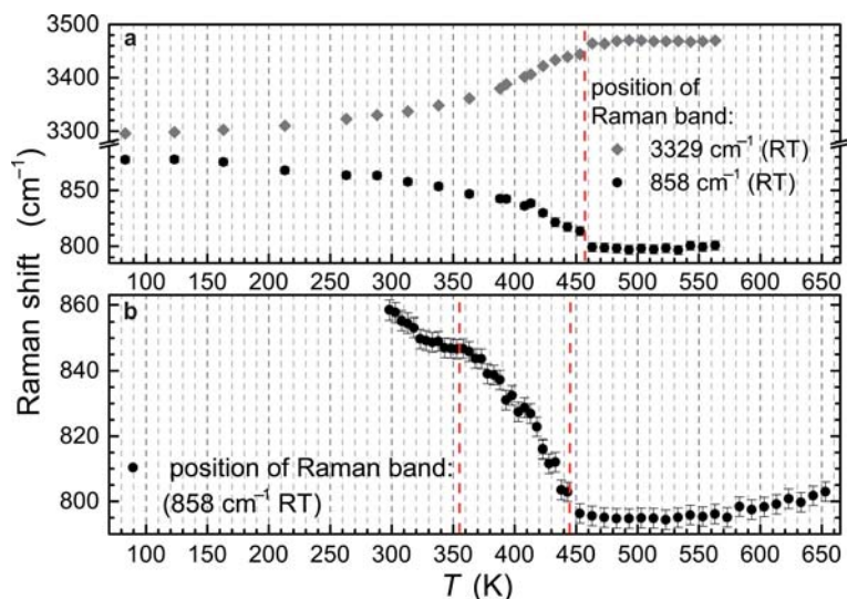
FIG. 5. Band shift analysis of two Raman bands. The band at 858 cm -1 (RT) is assigned to an out-of-plane bending vibration of the hydroxyl group and the band at 3329 cm -1 to a stretching vibration of the OH group. The lower plot shows two, clear, non-uniform changes, one around 355 K and the other around 445 K. The temperature behaviour of (a) and (b) is slightly different, possibly caused by the use of a single crystal (a) and Pb-lawsonite powder (b) for analysis.
