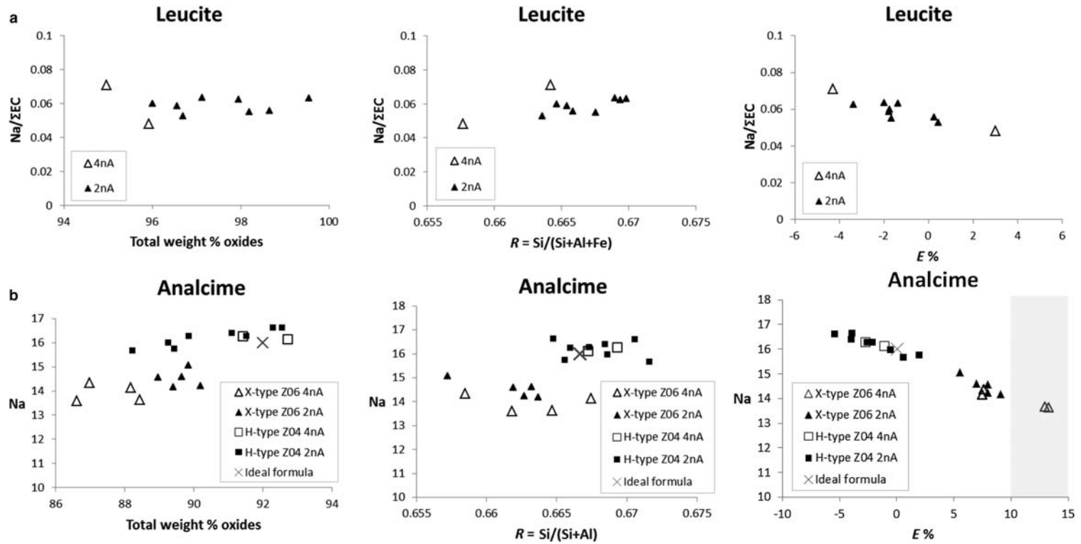
FIG. 3. Test 3: Effect of beam current on analyses of different reference zeolites. Total wt.% oxides exclude H_2O . \Sigma EC = sum of extraframework cations. Areas outside of the acceptable range of E\% (Passaglia, 1970), are shaded.
