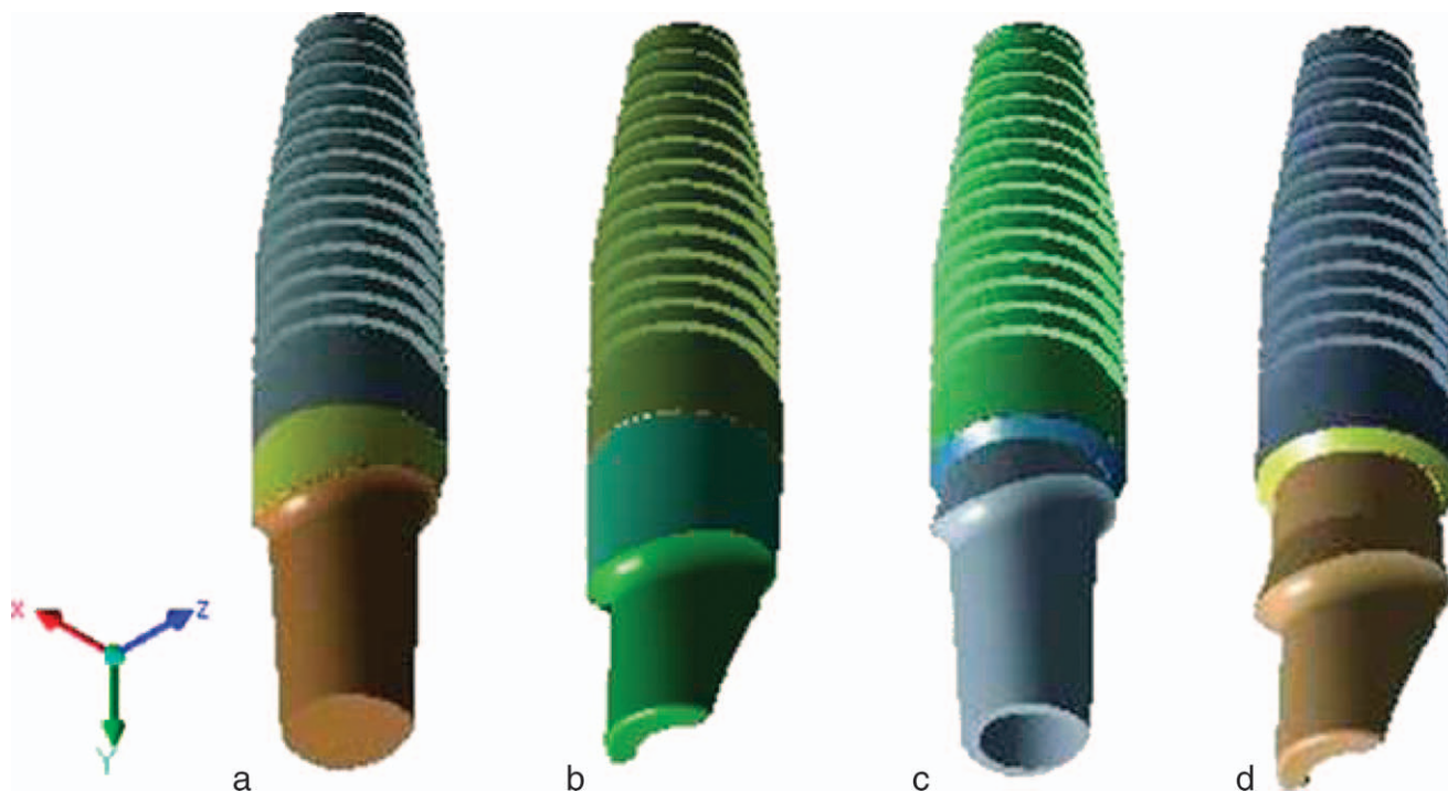
FIGURE 1. Models illustrating implants connected to straight and angulated abutments on a regular and a switching platform. (a) Regular platform and straight abutment. (b) Regular platform and angulated abutment. (c) Platform switching and straight abutment. (d) Platform switching and angulated abutment.
