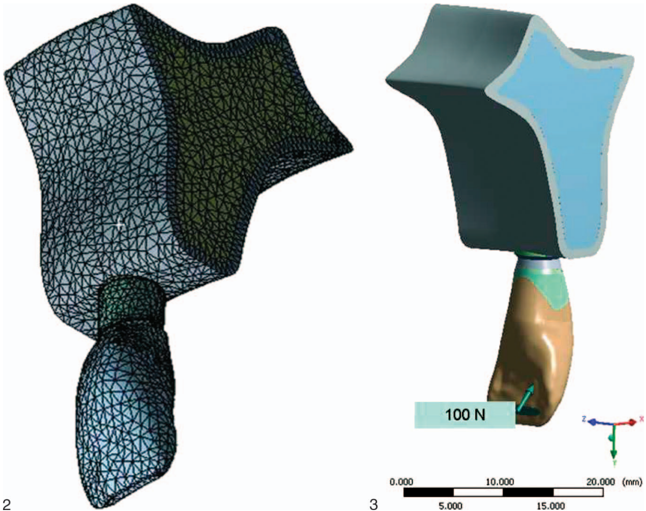
FIGURES 2 AND 3. FIGURE 2. Completed model with finite element mesh. FIGURE 3. Model representing the application of the force in oblique direction on the lingual face of prosthetic crown.
