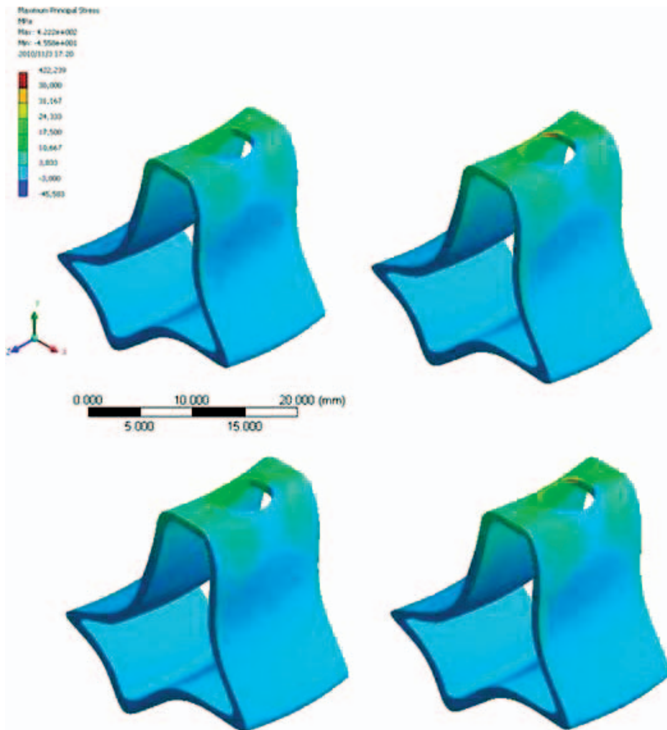
FIGURE 4. Maximum principal stress on cortical bone in models RS (regular platform and straight abutment), RA (regular platform and angulated abutment), SS (platform switching and straight abutment), and SA (platform switching and angulated abutment).
