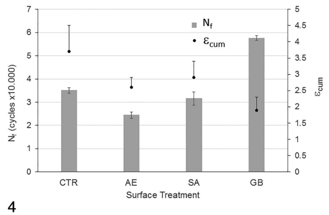
FIGURES 3 AND 4. FIGURE 3. Surface residual stresses calculated at the 4 different types of Ti dental implant surfaces, showing that the grit-blasted surface (GB) treatment provided the higher residual stress, whereas the other treatments provided similar residual stresses to that of as-received (CTR) samples. FIGURE 4. Fatigue test results, showing the number of cycles needed for failure (N f ) (left axis) and the cumulative plastic strain (ε cum ) (right axis) for the different treated surfaces. AE indicates acid-etched; SA, spark-anodization.
