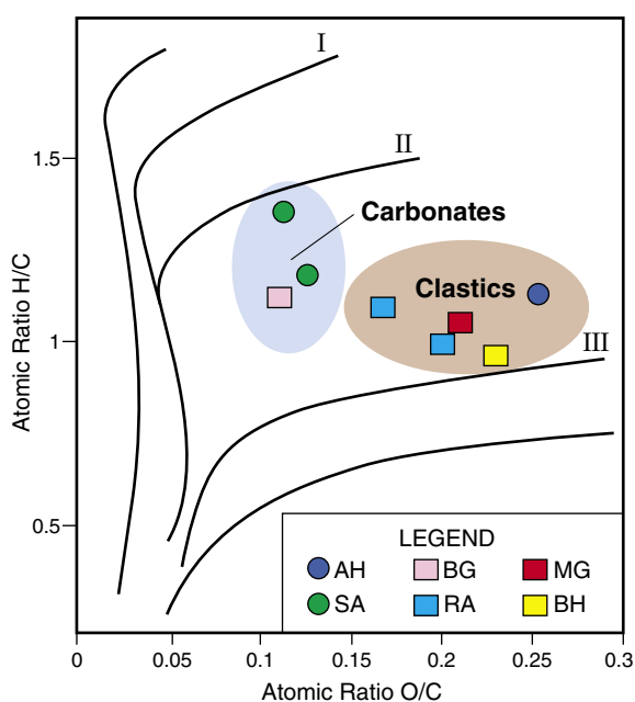
Figure 10: Geochemical characteristics of the insoluble organic matter.
