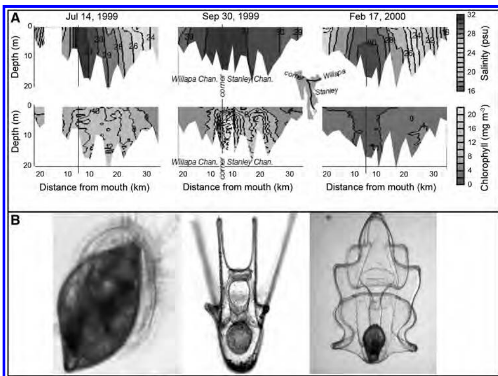
Figure 2. (A) Estuarine circulation and changes with time showing instantaneous vertical sections of salinity and chlorophyll along the Willapa (northern) and Stanley (southern) channels (in Willapa Bay, WA) from CTD transects on three dates. Students were asked to identify possible mechanisms that led to the observed differences in salinity and chlorophyll. Taken from Banas et al. (2007). (B) Images of meroplanktonic invertebrate larvae (meroplankton are organisms that spend only a part of their life in the water column): (left) a geoduck veliger (© Karen Chan); (middle) a sea star bipinnaria (© Fernanda Oyarzun); and (right) a sand dollar pluteus (© Karen Chan).
