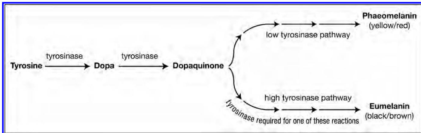
Figure 3. Schematic diagram of the pathway of melanin synthesis. All melanin is made from the amino acid tyrosine. When tyrosinase levels are low, pheomelanin (yellow/red) is produced; when tyrosinase levels are high, eumelanin (black/brown) is produced. Individuals completely lacking in tyrosinase make no melanin of any kind and are albino. Albinism is most frequently caused by a mutation in the gene coding for tyrosinase (OMIM no. 606933).
