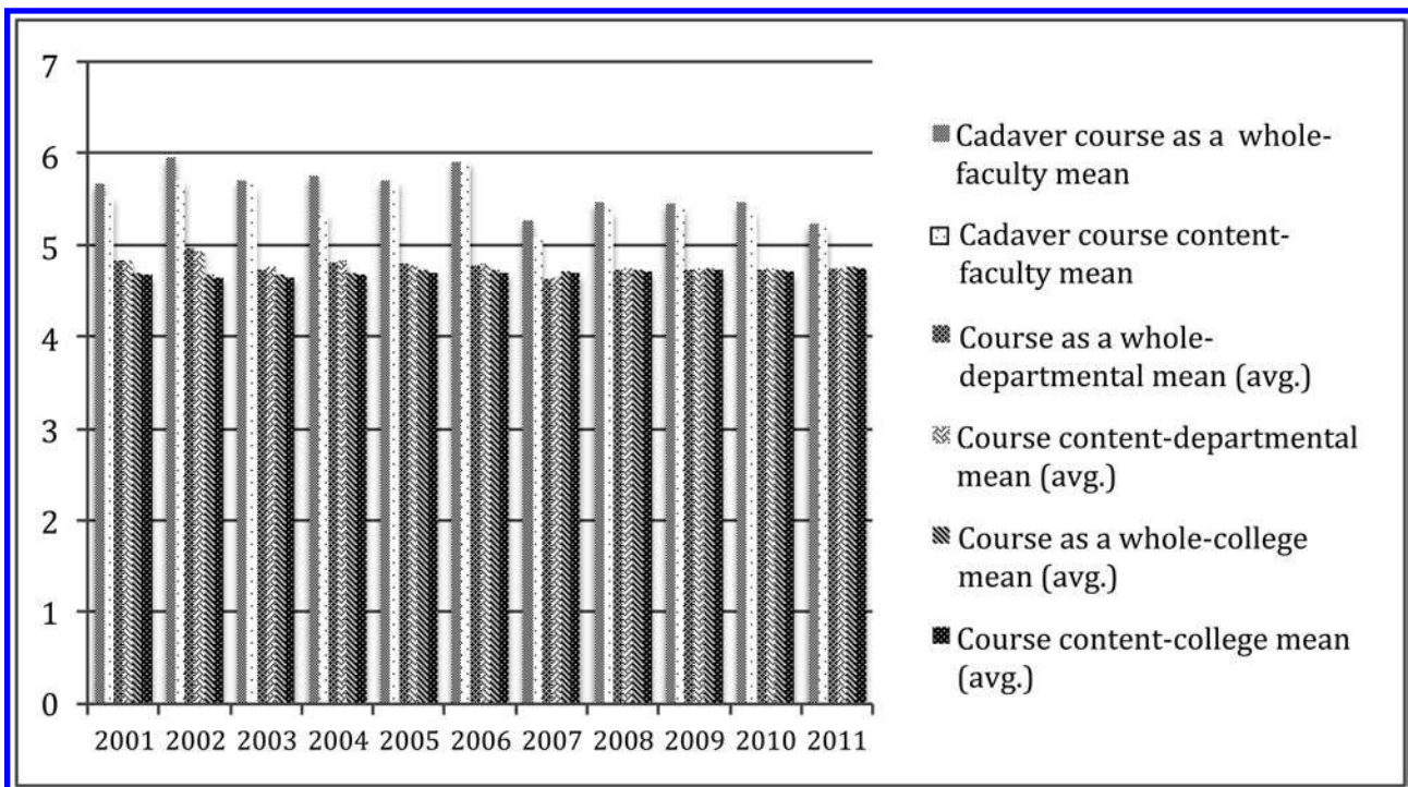
Figure 2. Departmental and university course comparisons against the cadaver course during the same year in two major categories.
