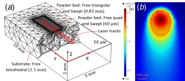
Fig. 2 (a) powder bed and substrate with selective meshing scheme. (b) surface temperature distribution at t = 0.14 \text{ s} . The lined isotherm indicates T = T_m .
