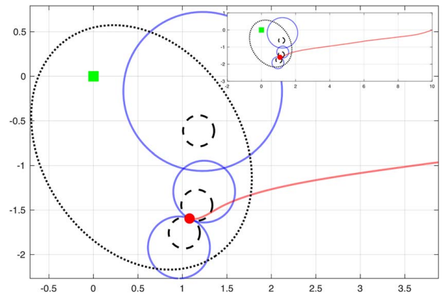
Fig. 3 Example scenario for N=3 . All simulations were performed for \sigma = 0.5 , \varepsilon = 0.175 , \bar{v}_e = 1 , and t_f = 15 . The defended area is given by the green box at (0, 0) . The blue circle corresponds to the capture set approximation in (16), whose center is the desired quantity to be controlled, and the black dashed circle shows the capture distance for each individual pursuer. The red curve corresponds to the evader trajectory, and the dotted ellipse corresponds to the evader's constrained reachable set. Note how the evader tries to maneuver between the bottom two pursuers, but ultimately enters the capture region.
