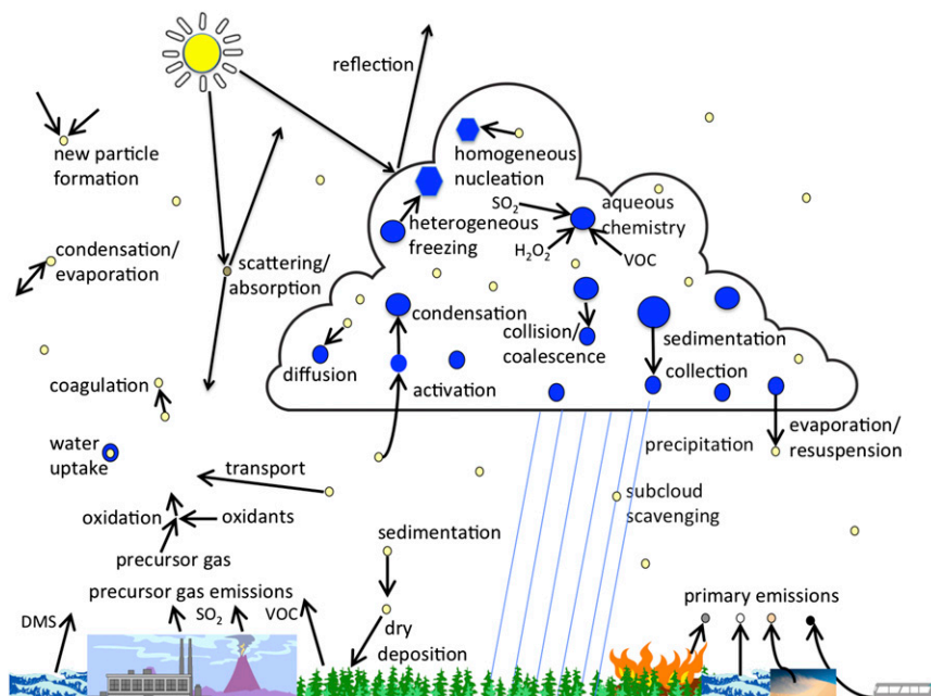
FIG. 27-1. Atmospheric processes important for producing aerosol effects on climate (after Ghan and Schwartz 2007).
