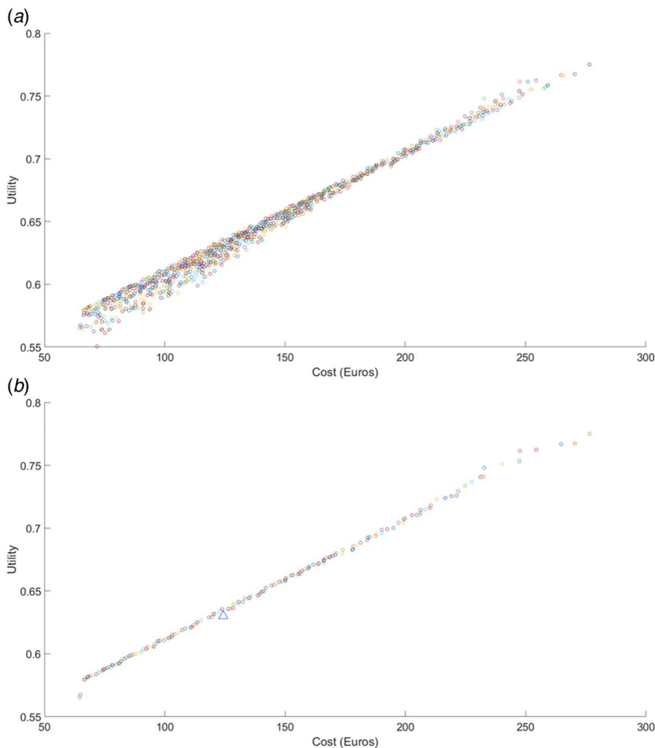
Fig. 8 Optimization study results—(a) Tradespace analysis result for Design Aspect B, and (b) Selected optimal designs with original E. Howard design shown in the \Delta symbol.
