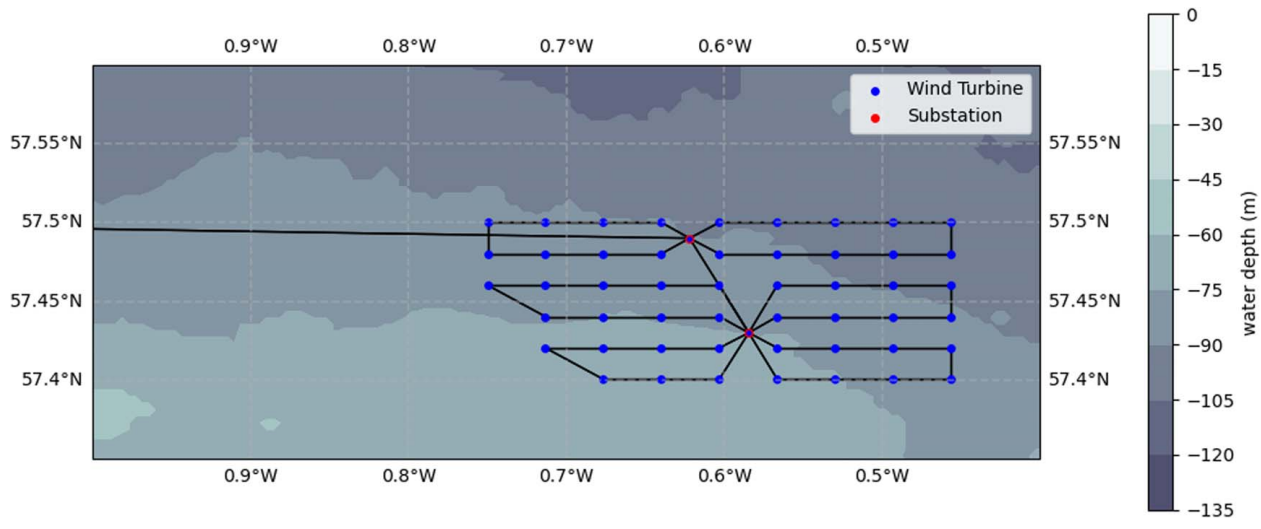
Fig. 5 Floating wind farm layout with 50 single 14 MW turbines
