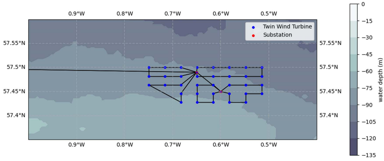
Fig. 4 Floating wind farm layout with 35 twin 10 MW turbines
