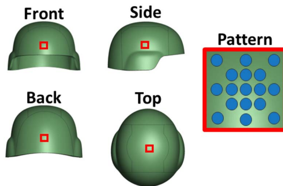
Fig. 4 Impact pattern and position for each helmet orientation
