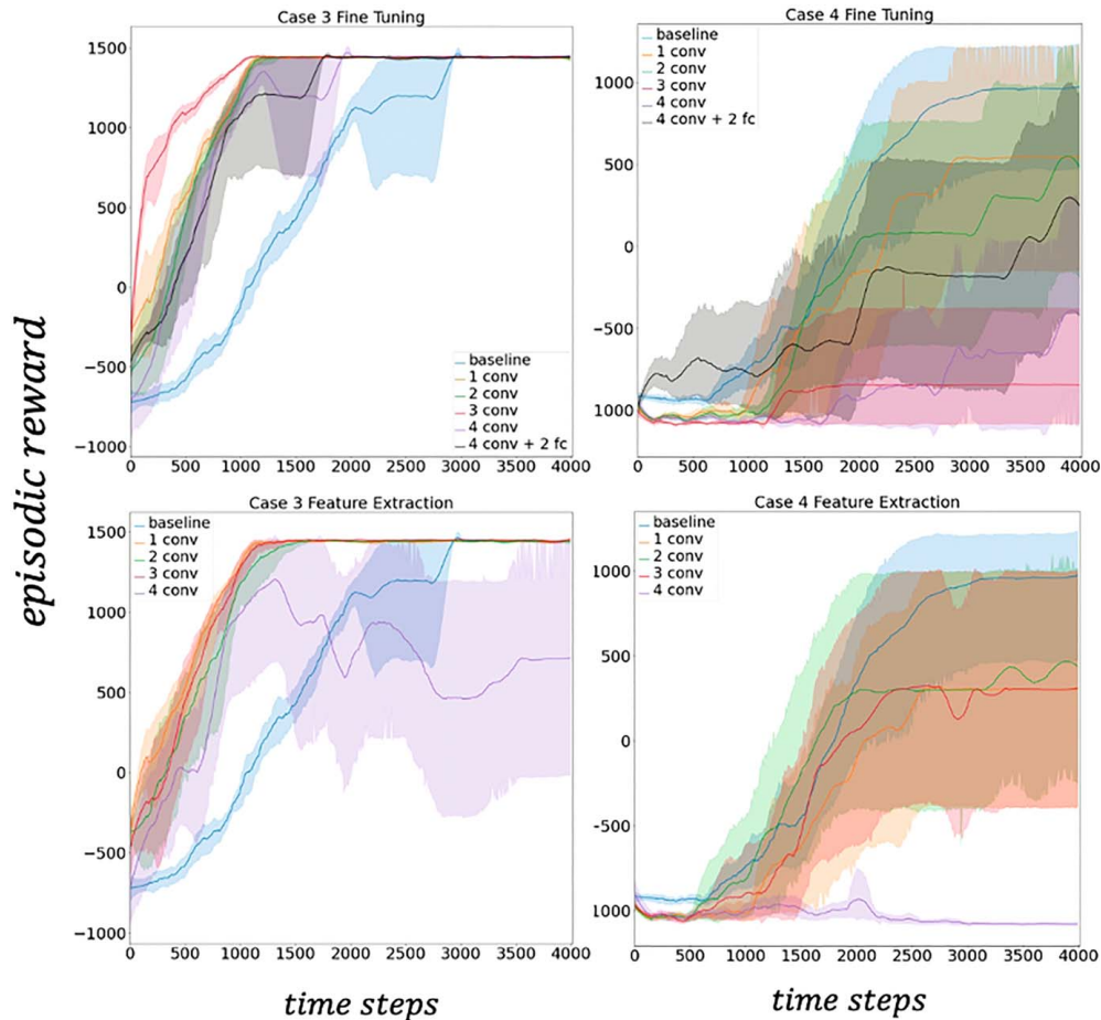
Fig. 8 Reward of case 3 and case 4 using the different layer-level transfer learning strategies
