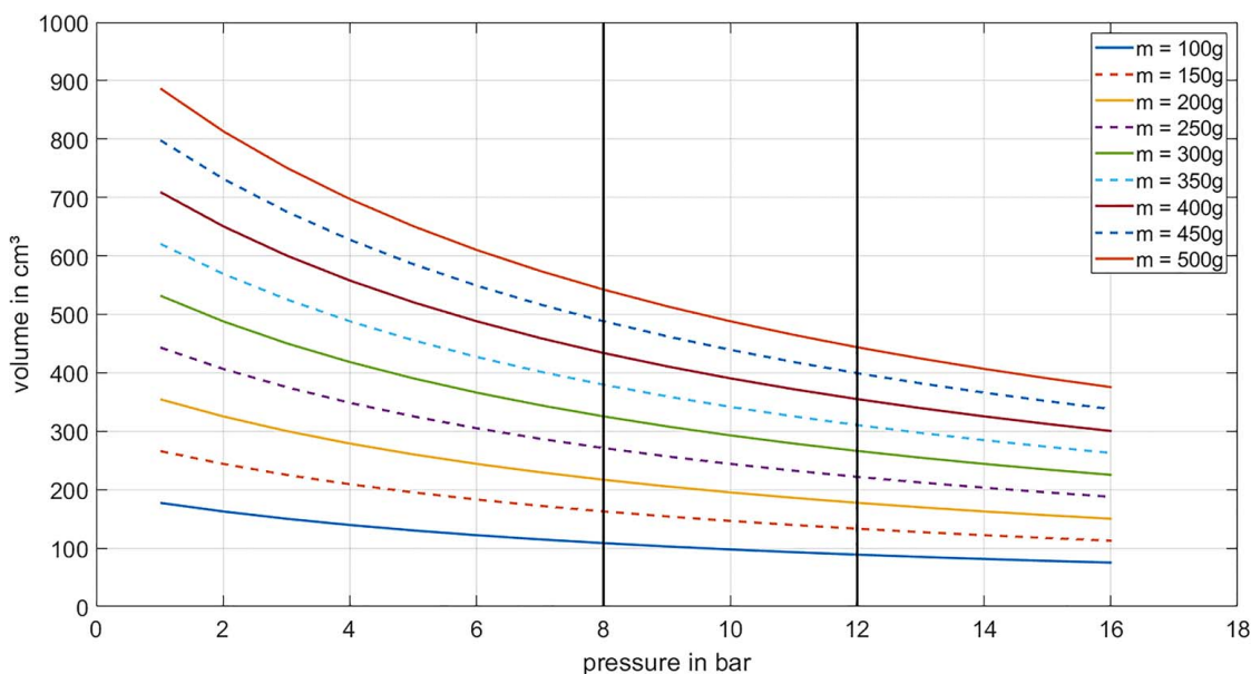
Fig. 9 Set of curves for volume savings
