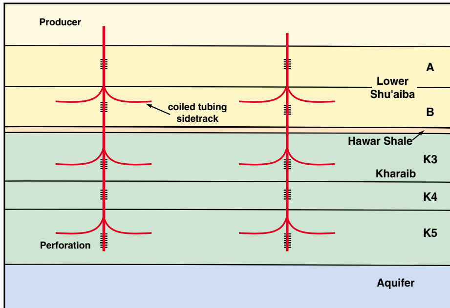
Figure 6a: Short horizontal side-tracks from vertical stem well.
